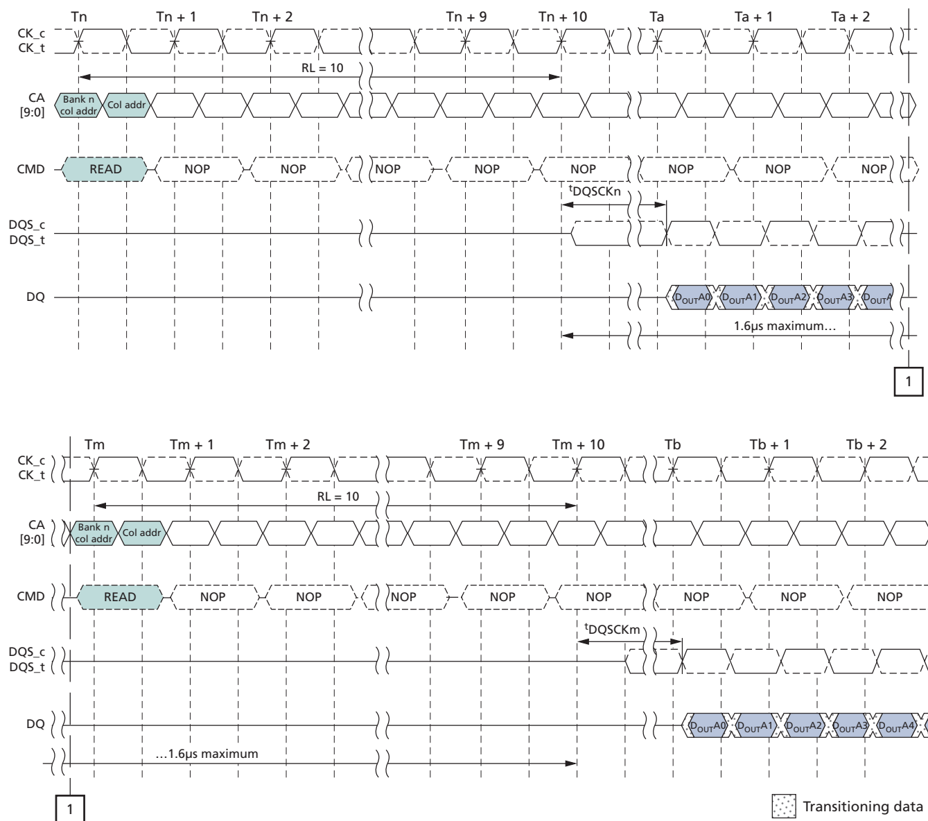
Figure 23: t_{DQSKDM} Timing
