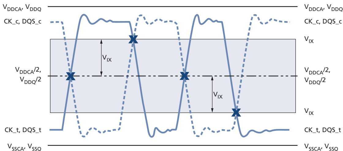
Figure 76: V_{IX} Definition
