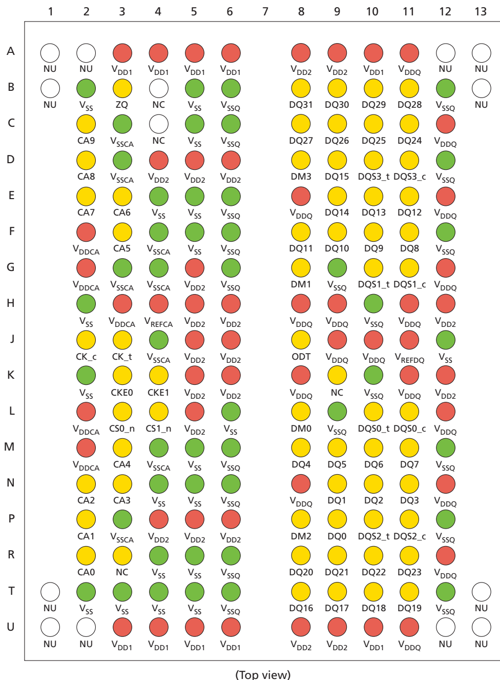
Figure 3: 178-Ball Single-Channel FBGA – 2 x 8Gb Die
