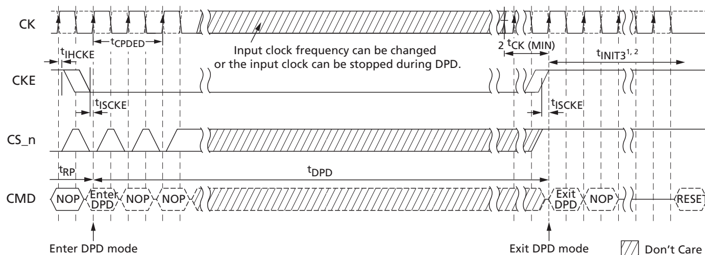
Figure 70: Deep Power-Down Entry and Exit Timing
