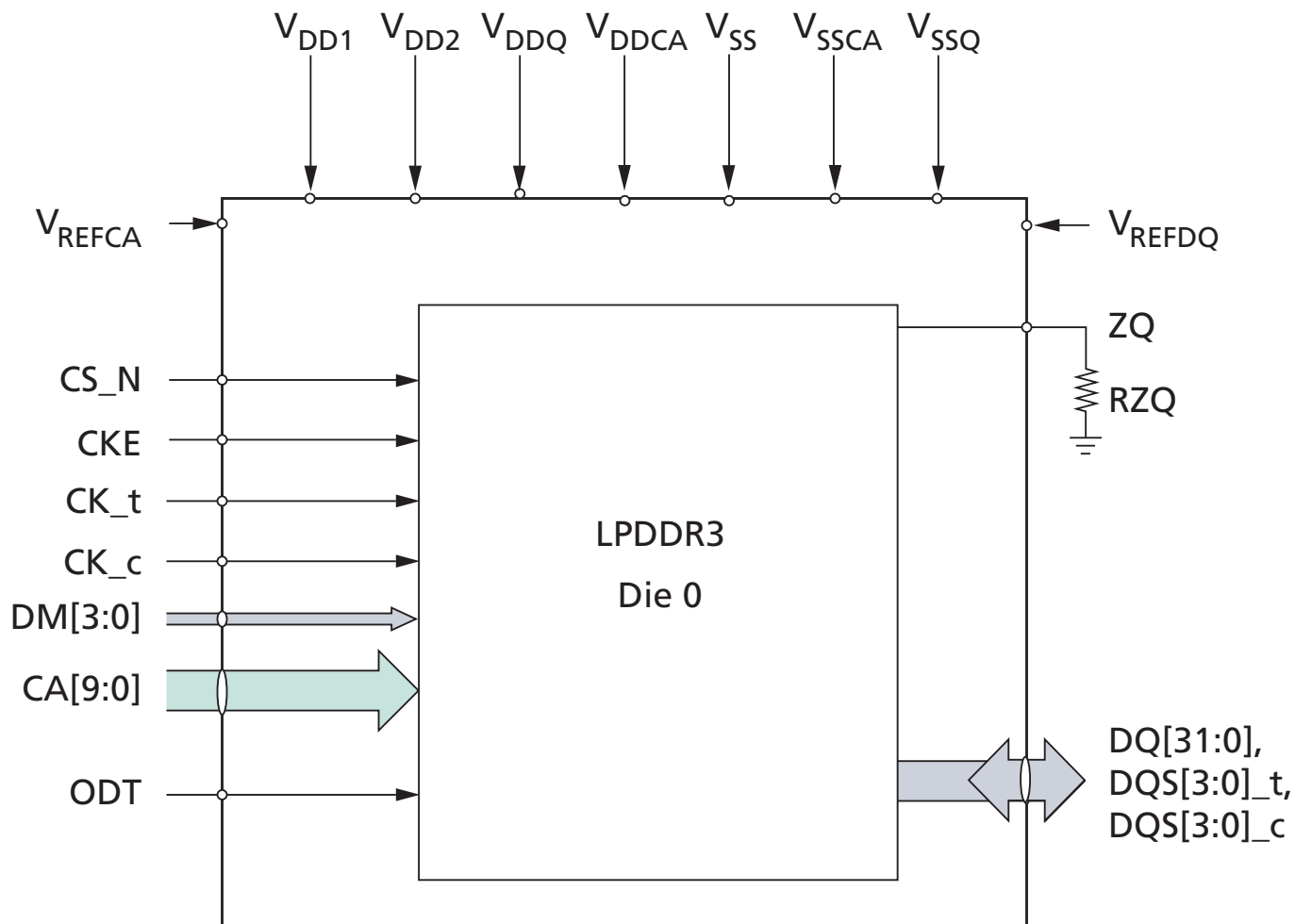
Figure 5: Single-Die, Single-Channel Package Block Diagram
