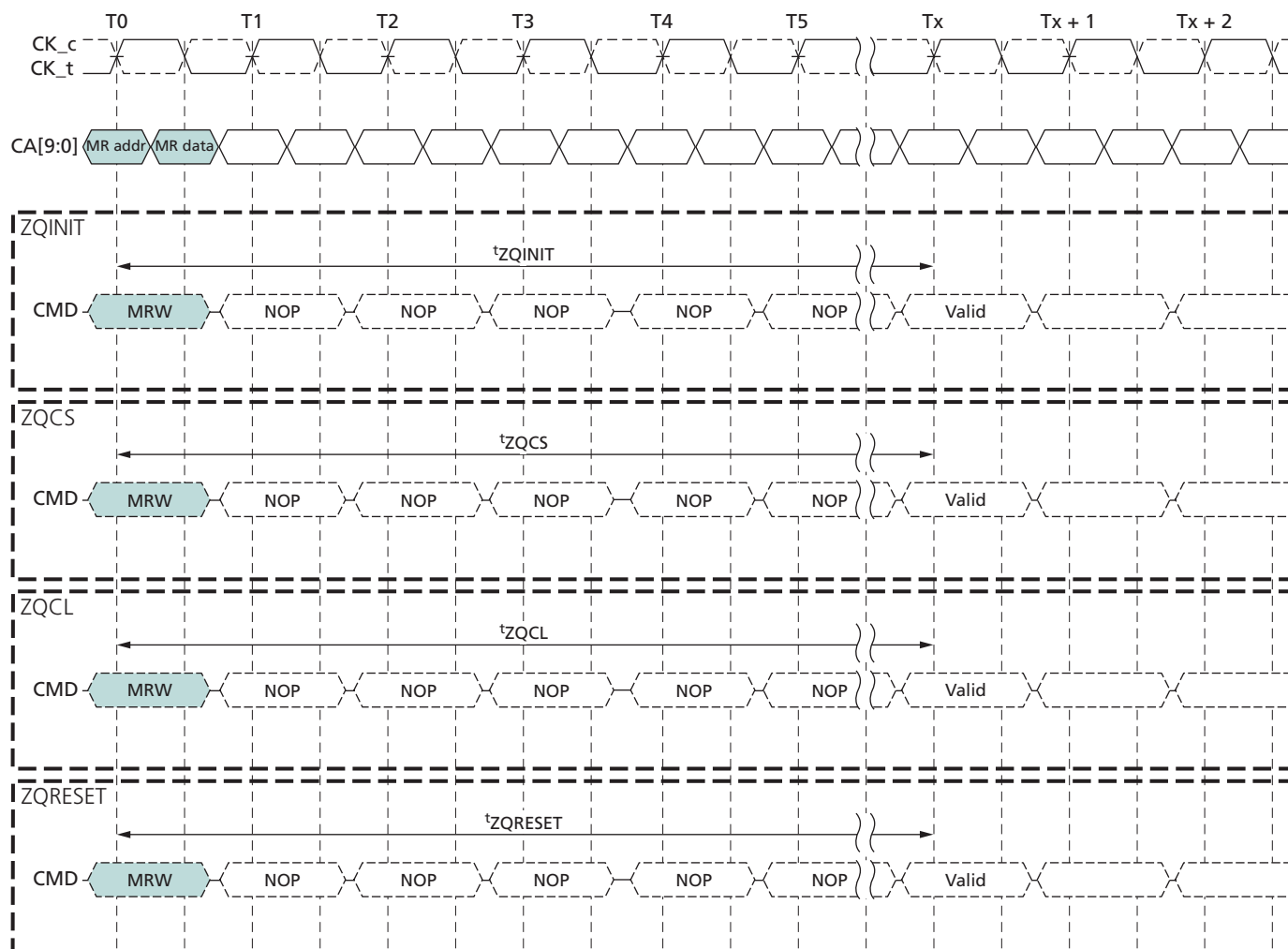
Figure 51: ZQ Timings
