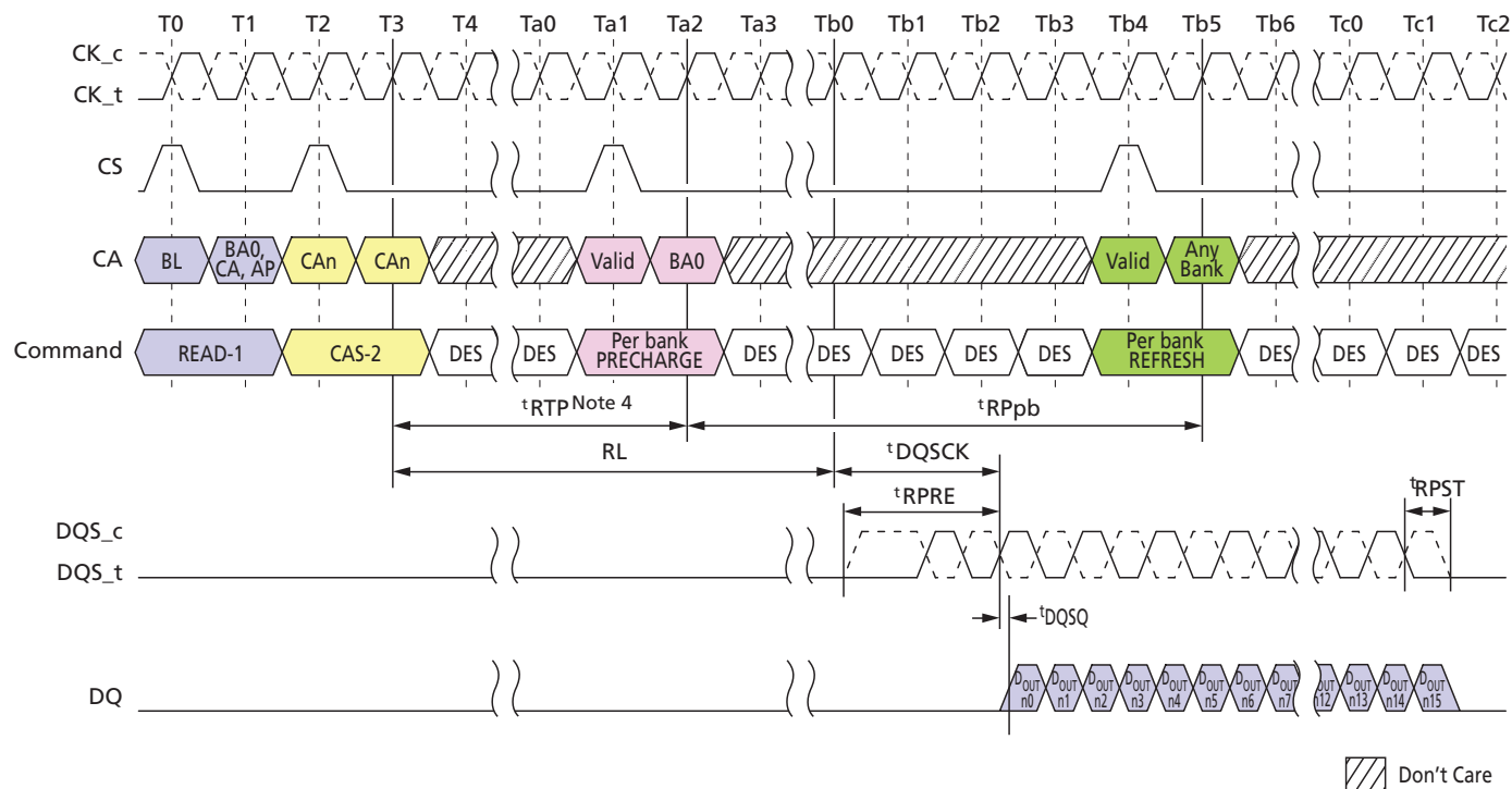
Figure 73: Burst READ Operation Followed by Per Bank Refresh
