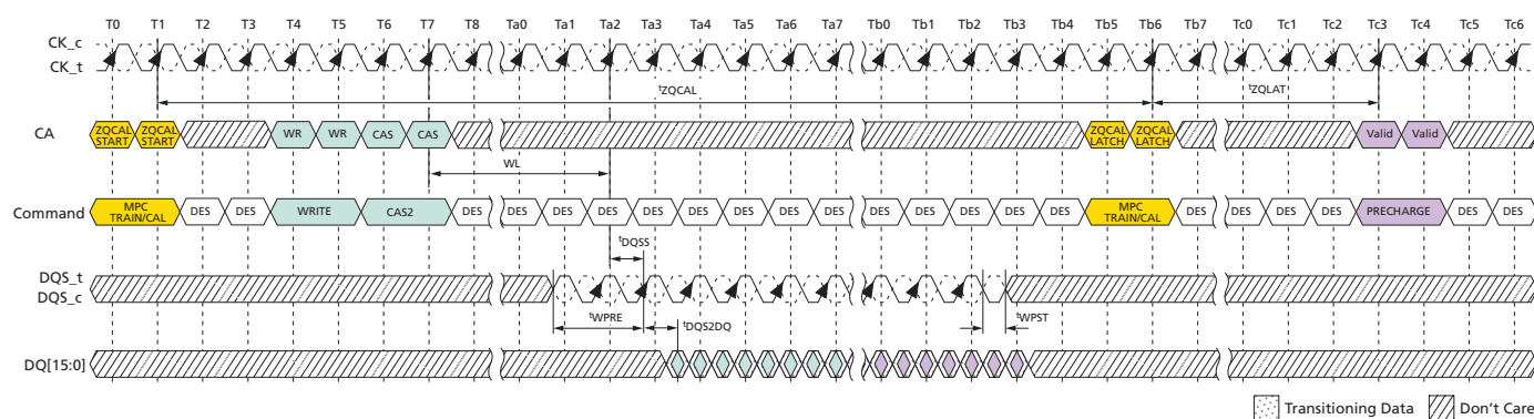
Figure 134: ZQCAL Timing
