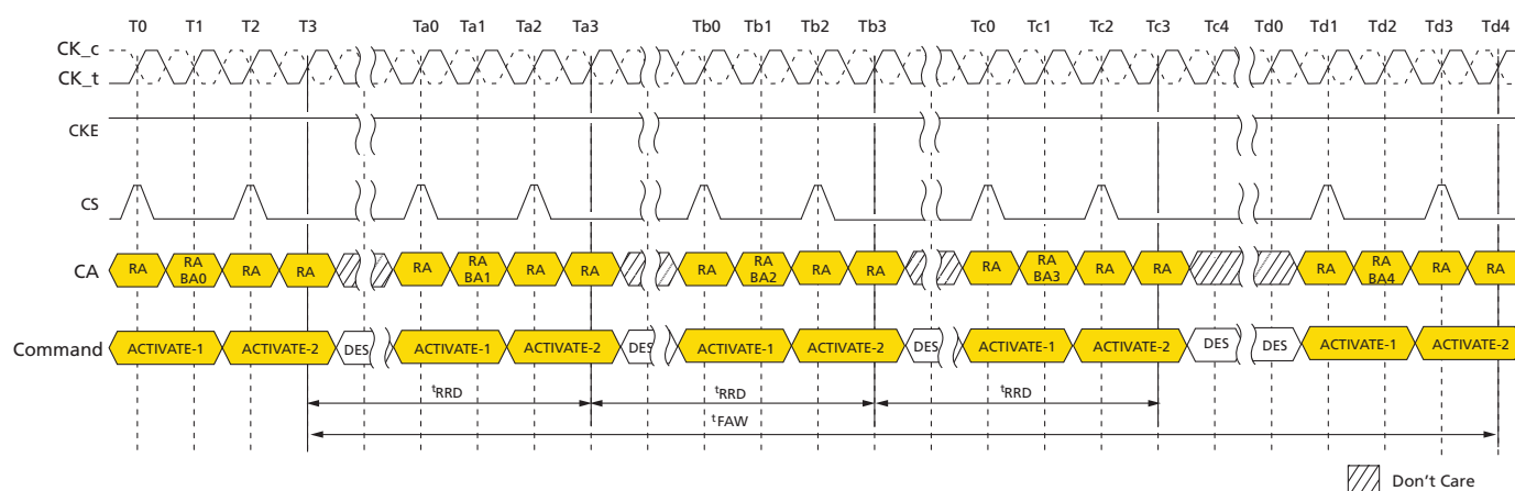
Figure 12: t_{FAW} Timing
