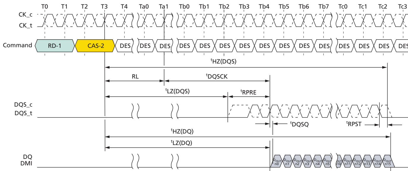
Figure 20: Read Timing
