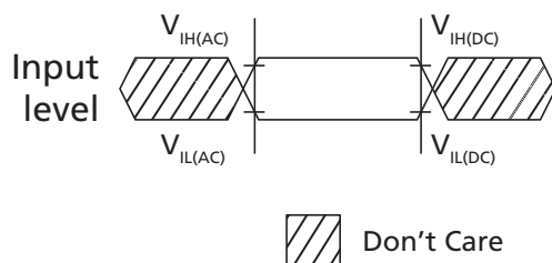
Figure 146: Input Timing Definition for CKE
