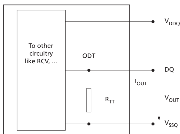
Figure 141: Functional Representation of DQ ODT
