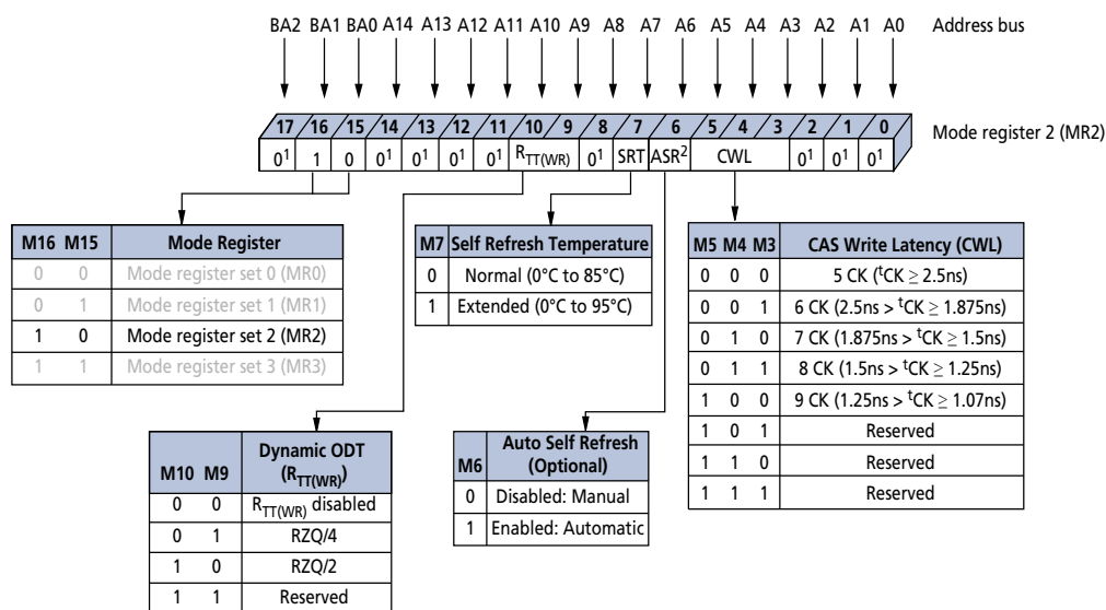
Figure 56: Mode Register 2 (MR2) Definition
