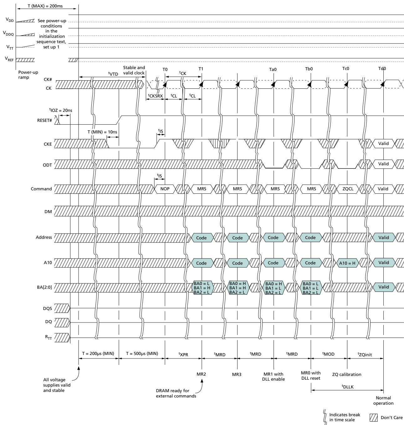
Figure 49: Initialization Sequence
