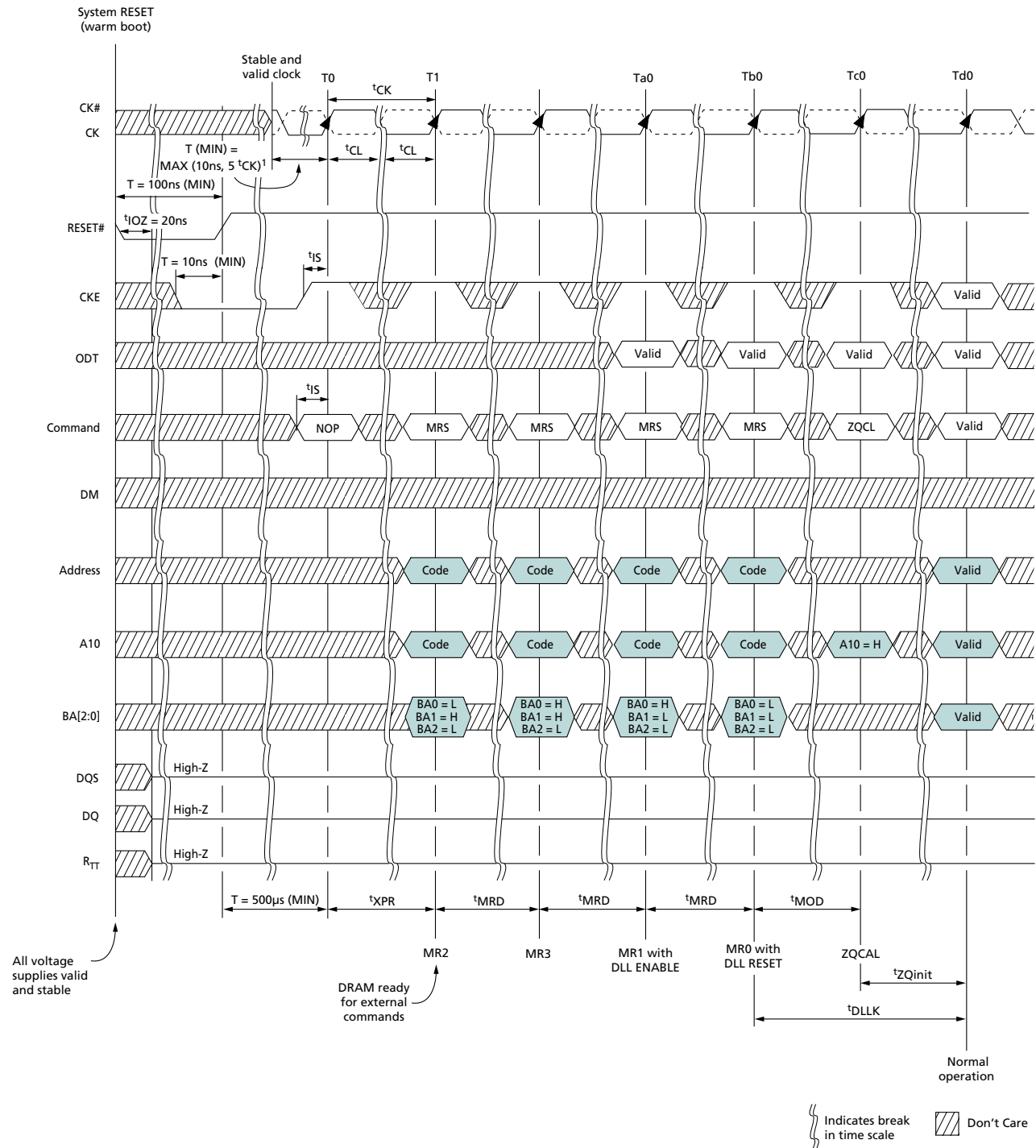
Figure 107: RESET Sequence
