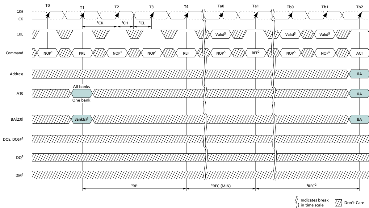
Figure 41: Refresh Mode
