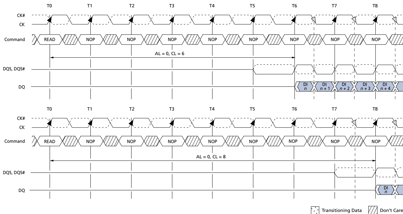
Figure 53: READ Latency
