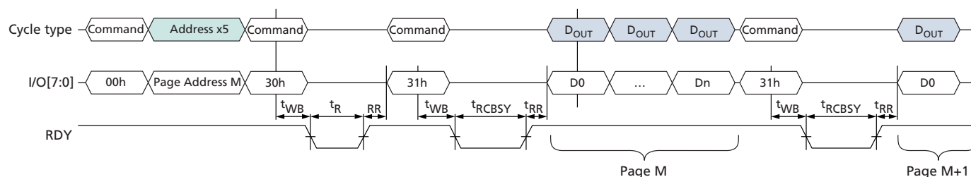
Figure 32: READ PAGE CACHE SEQUENTIAL (31h) Operation
