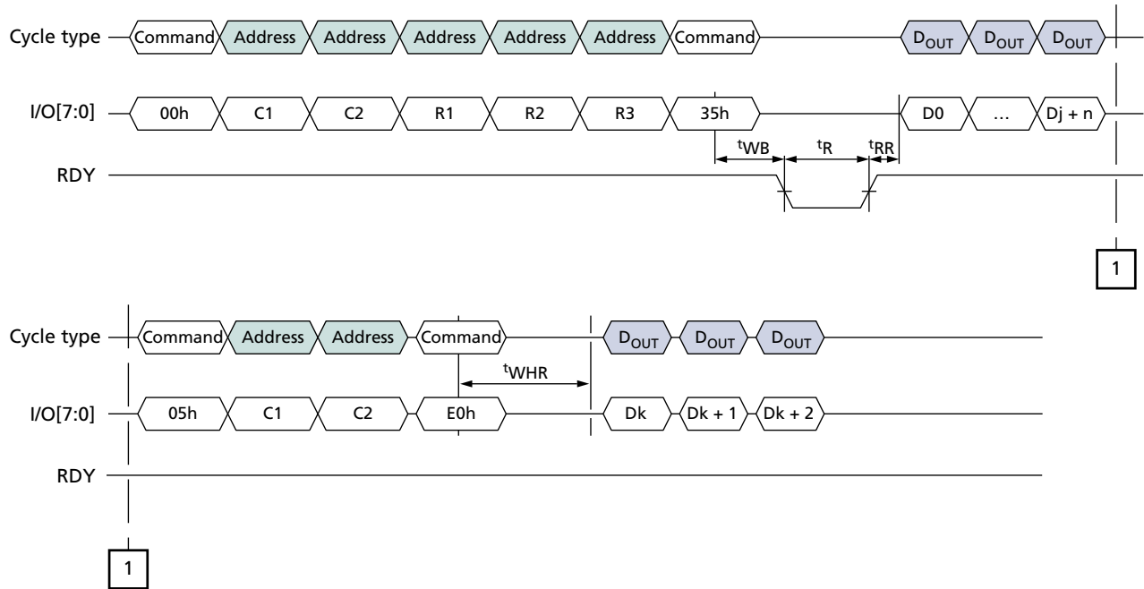
Figure 40: READ FOR INTERNAL DATA MOVE (00h–35h) with RANDOM DATA READ (05h–E0h)
