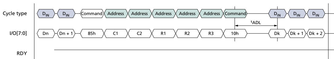
Figure 29: PROGRAM FOR INTERNAL DATA INPUT (85h) Operation
