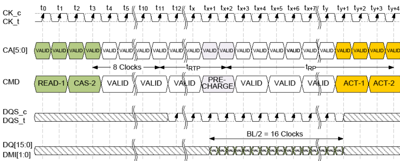
Burst READ followed by PRECHARGE (Shown with BL32, 2tCK pre-ambble)
