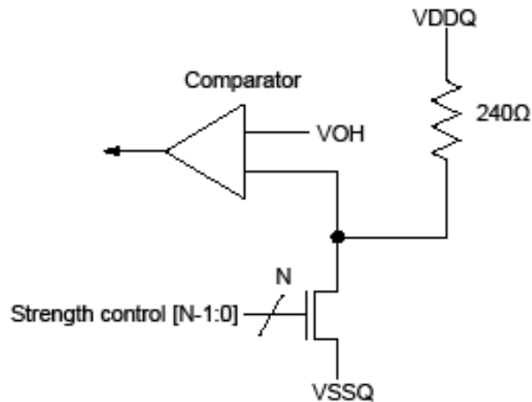
pull-down calibration
