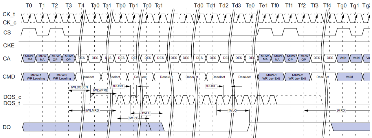
Write Leveling Timing, tDQSL(min)
