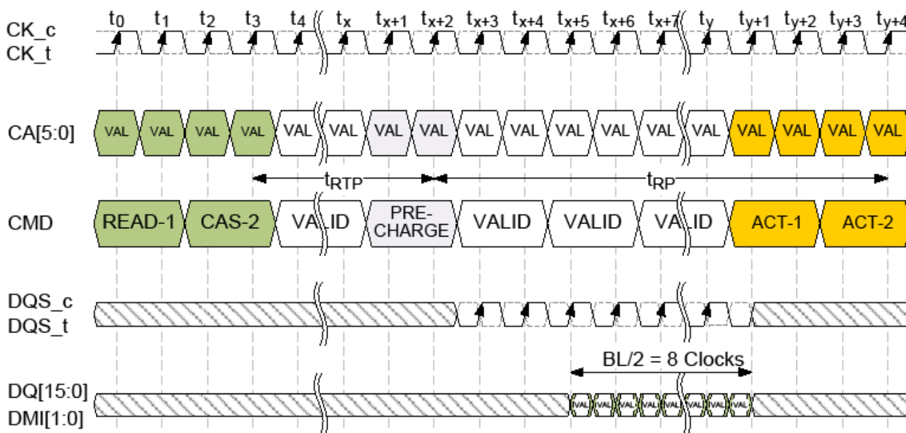
Burst READ followed by PRECHARGE (Shown with BL16, 2tCK pre-ambble)
