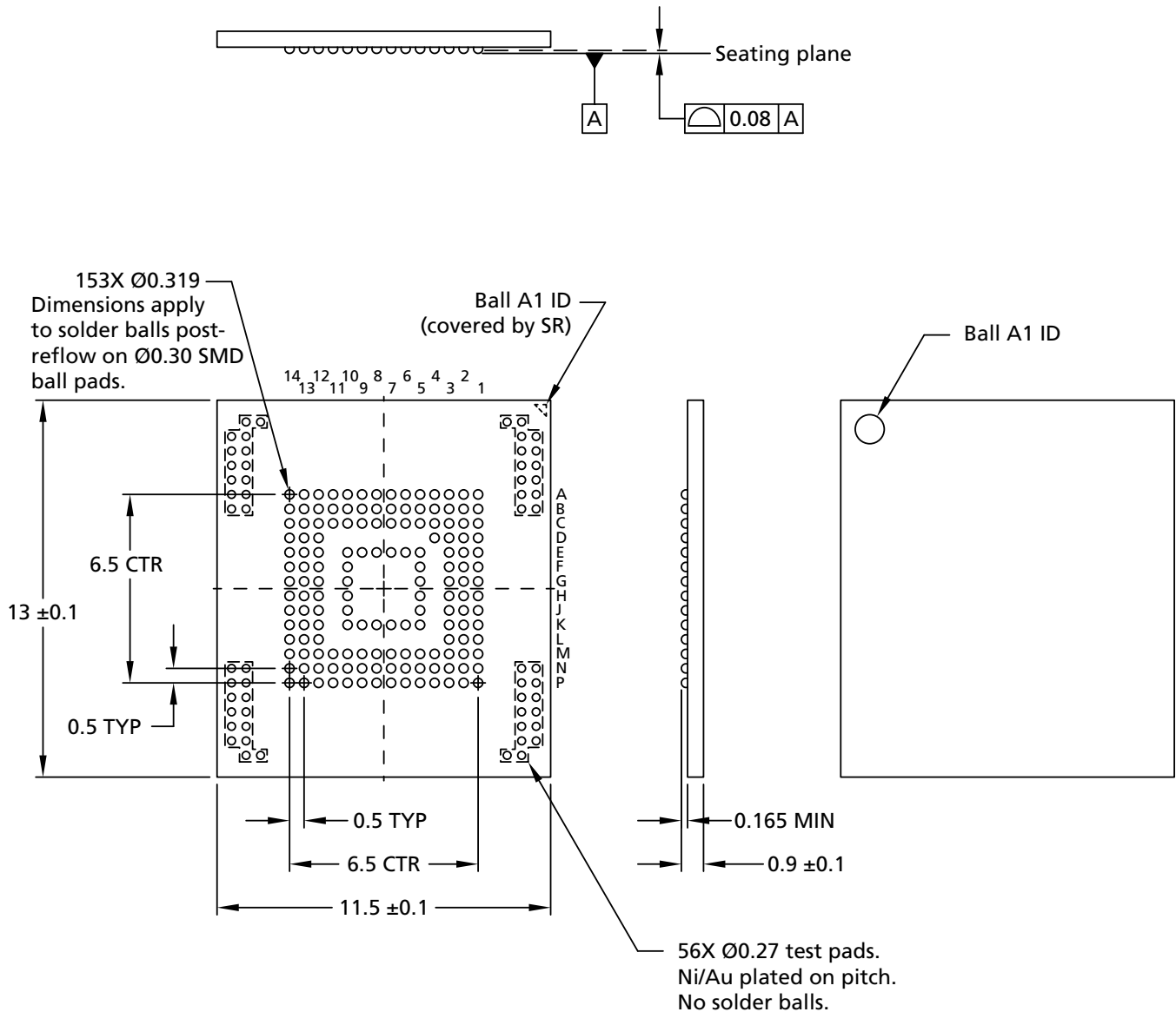
Figure 6: 153-Ball VFBGA – 11.5mm x 13.0mm x 1.0mm (Package code AM)
