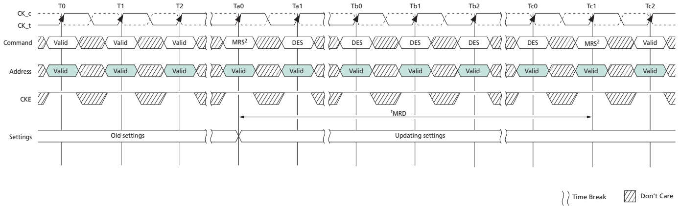
Figure 8: t^{\text{MRD}} Timing
