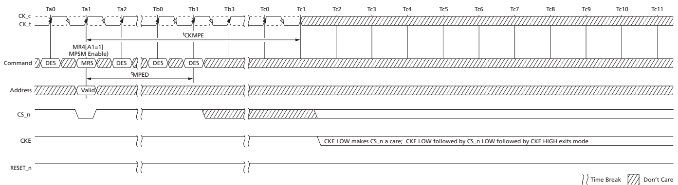
Figure 38: Maximum Power-Saving Mode Entry
