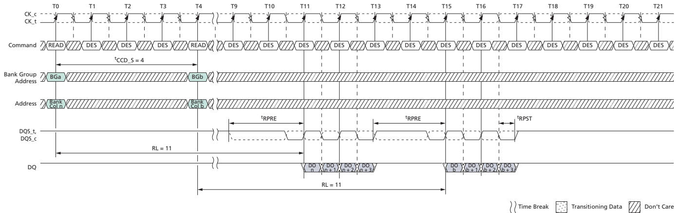
Figure 127: READ (BC4) to READ (BC4) with 2 nd CK Preamble in Different Bank Group
