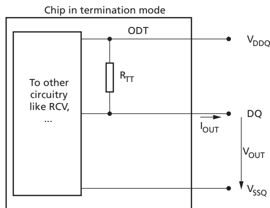
Figure 226: ODT Definition of Voltages and Currents
