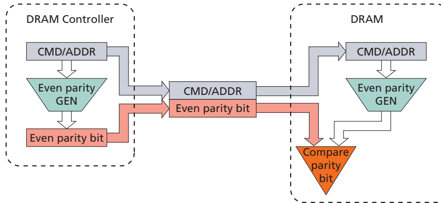
Figure 42: Command/Address Parity Operation
