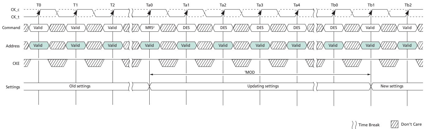
Figure 9: t^{\text{MOD}} Timing
