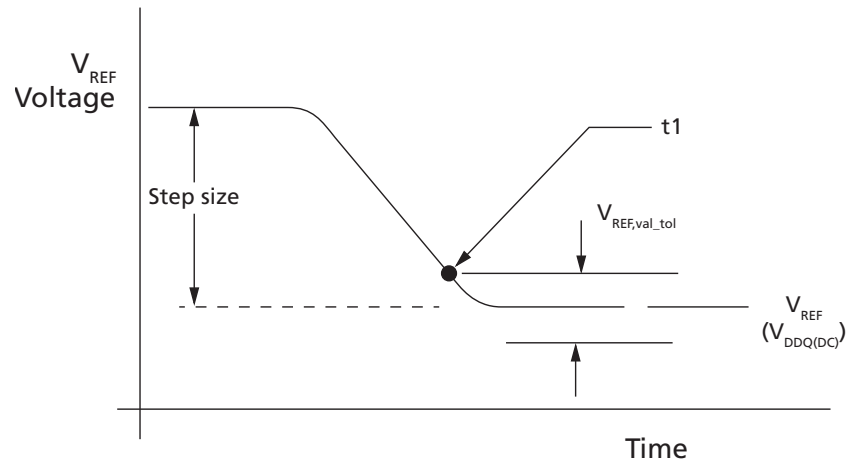
Figure 61: V REF Step: Single Step Size Decrement Case
