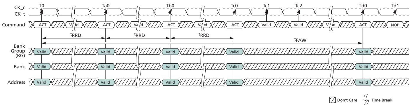
Figure 72: t_{FAW} Timing
