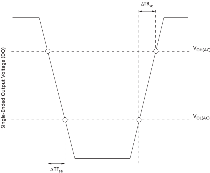
Figure 219: Single-ended Output Slew Rate Definition
