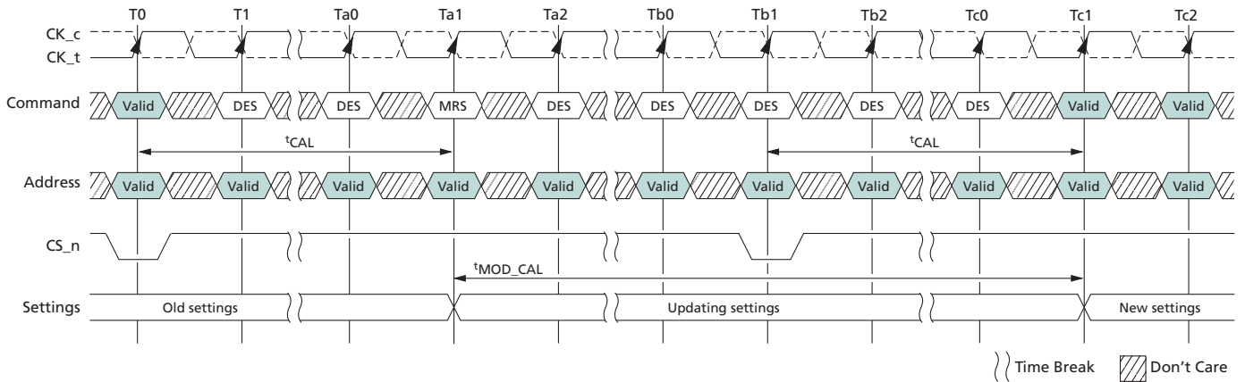
Figure 20: t_{MOD\_CAL} , MRS to Valid Command Timing with CAL Enabled
