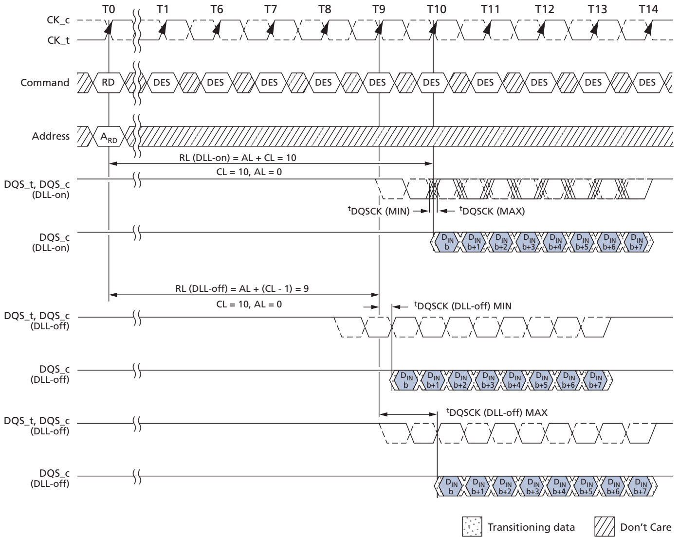
Figure 10: DLL-Off Mode Read Timing Operation
