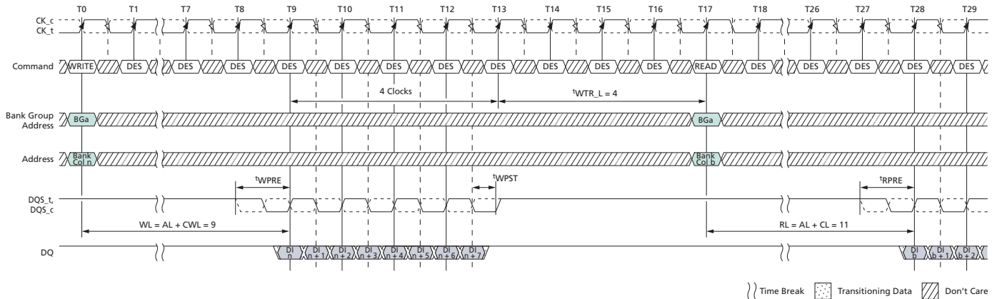
Figure 172: WRITE (BL8) to READ (BL8) with 1^t\text{CK} Preamble in Same Bank Group
