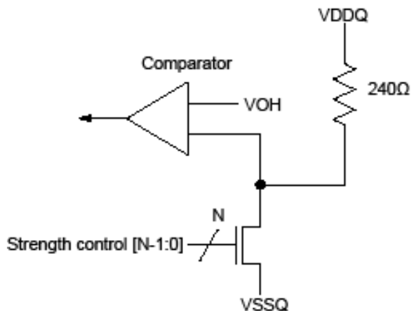
pull-down calibration
