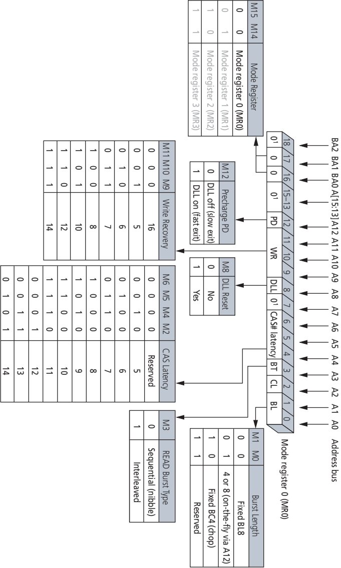
Figure 50: Mode Register 0 (MR0) Definitions
