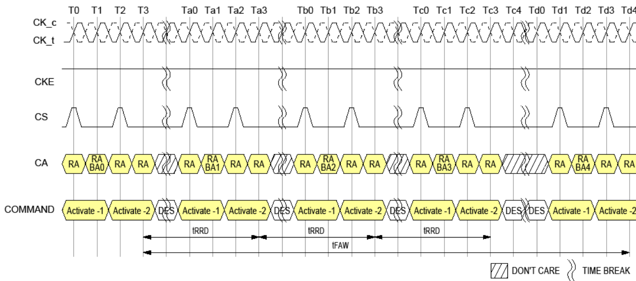
tFAW Timing
