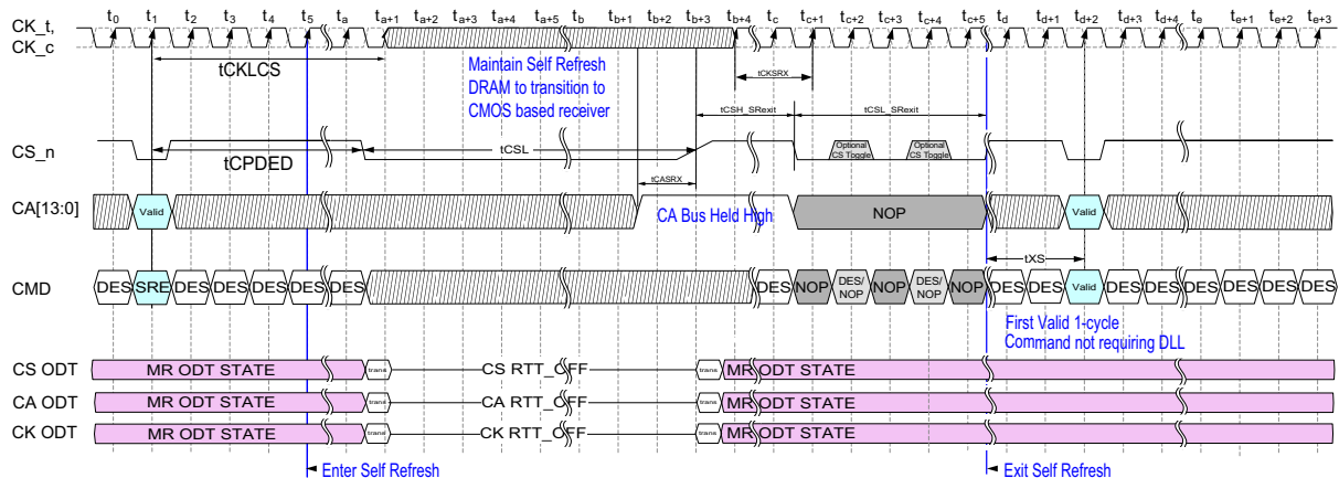
Figure 57 — Self-Refresh Entry/Exit Timing in 2N Mode w/ 1-Cycle exit command
