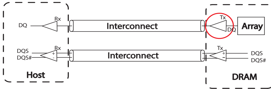
Figure 241 — Example of DDR5 Memory Interconnect
