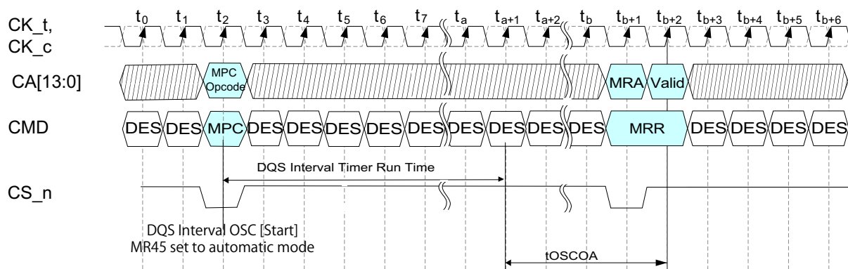
Figure 138 — DQS Interval Oscillator Automatic Mode Timing Diagram
