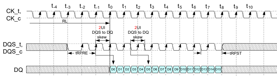
Figure 243 — Read burst example for pin DQx depicting bit 0 and 5 relative to the DQS edge for 2 UI skew with Read DQS Offset Timing set to 1 Clock (2UI)
