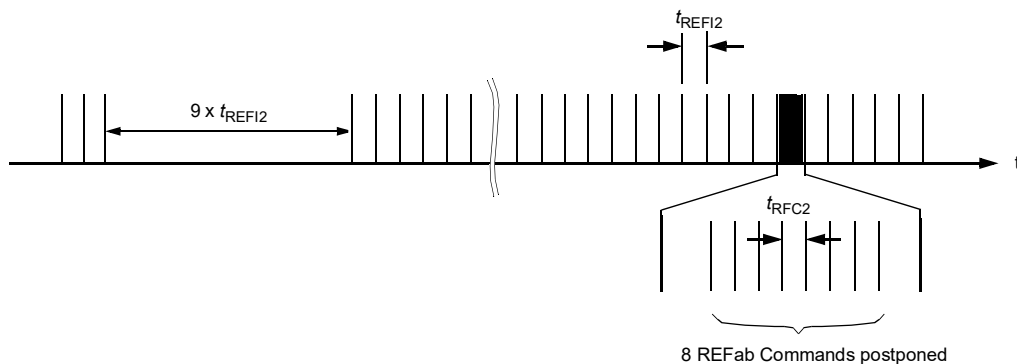
Figure 68 — Postponing Refresh Commands (Example of Fine Granularity Refresh Mode - t_{REFI2} , t_{RFC2} )
