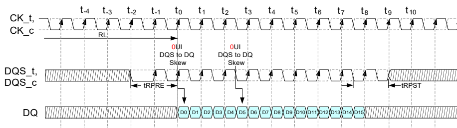
Figure 242 — Read burst example for pin DQx depicting bit 0 and 5 relative to the DQS edge for 0 UI skew
