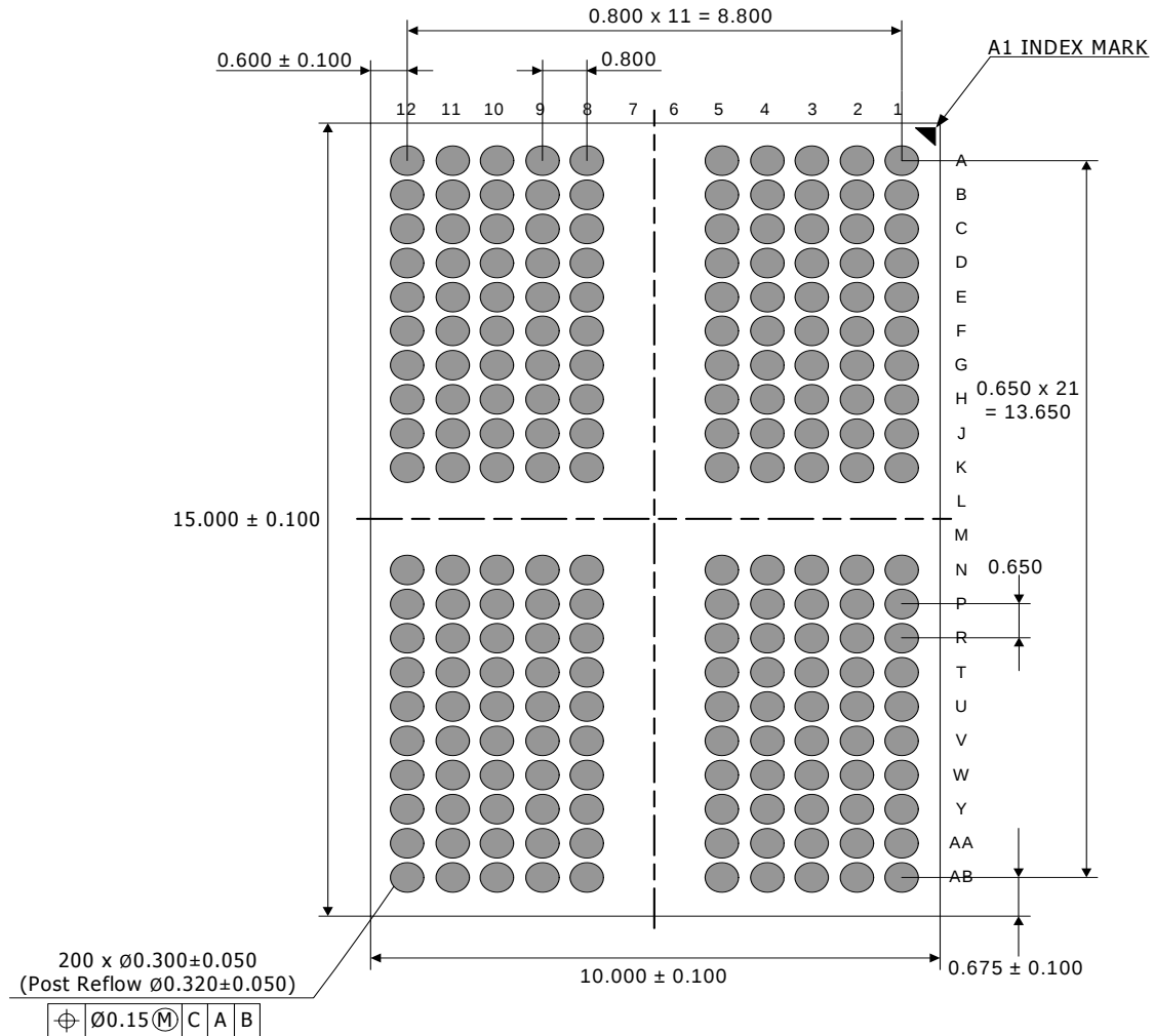
Bottom View
