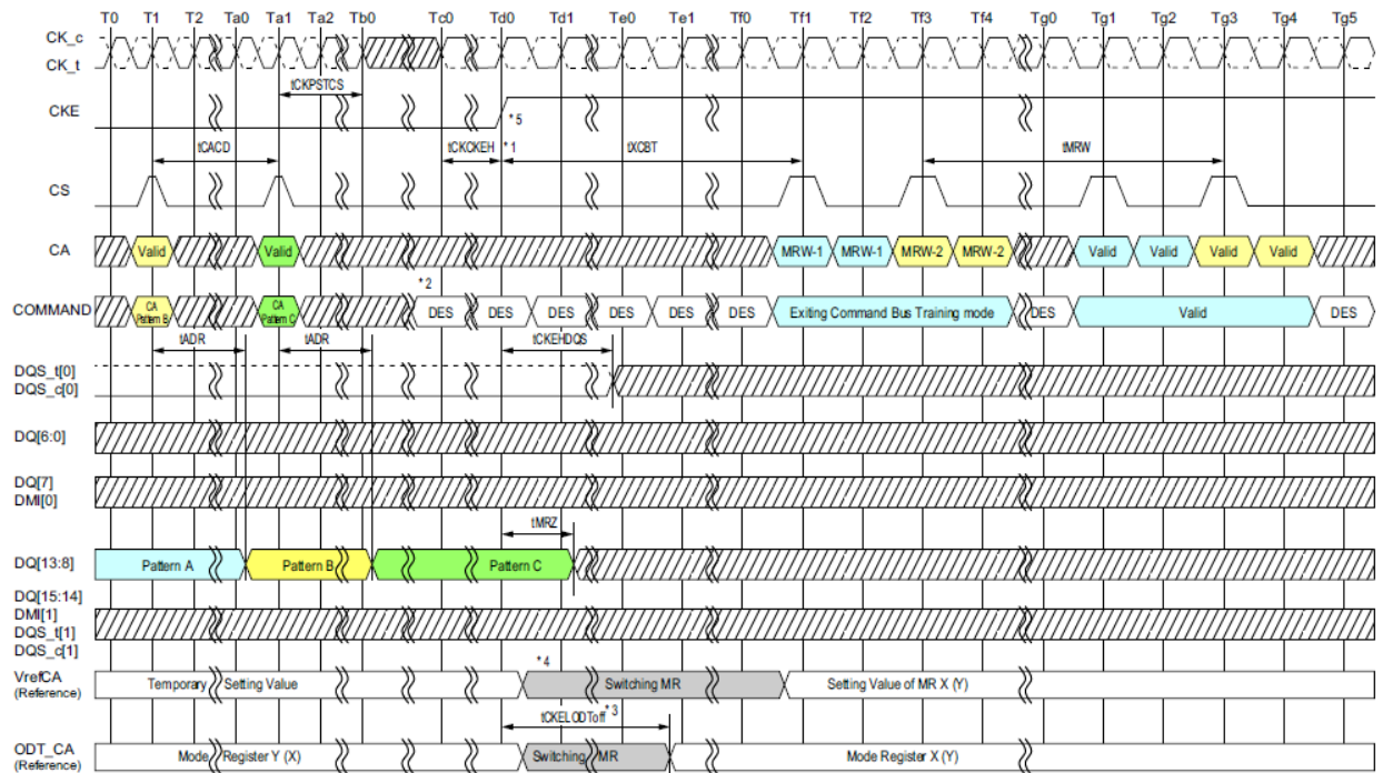
Figure - Exiting Command Bus Training Mode with Valid Command
