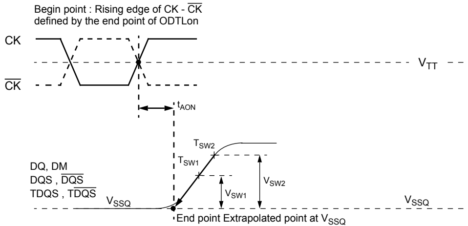
Figure 13. Definition of t_{\text{AON}}
