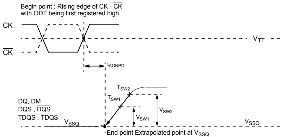
Figure 14. Definition of t_{\text{AONPD}}
