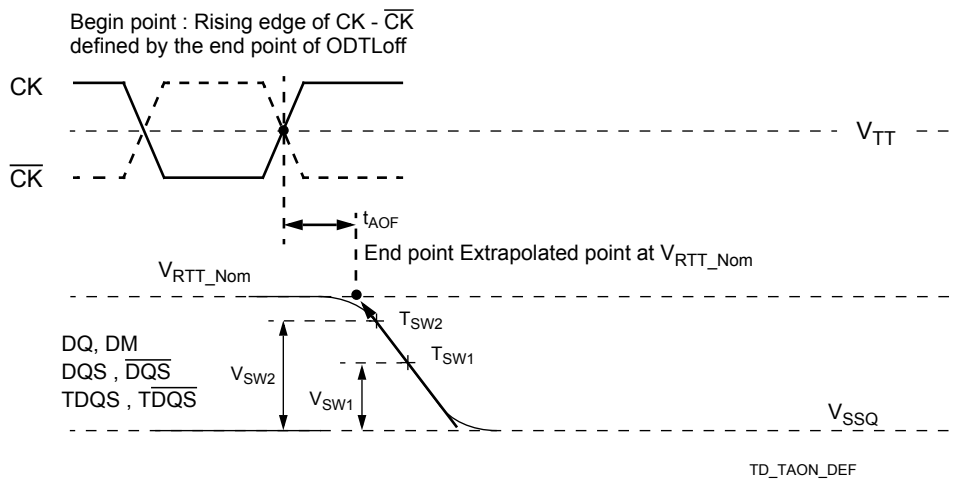
Figure 15. Definition of t_{\text{AOF}}
