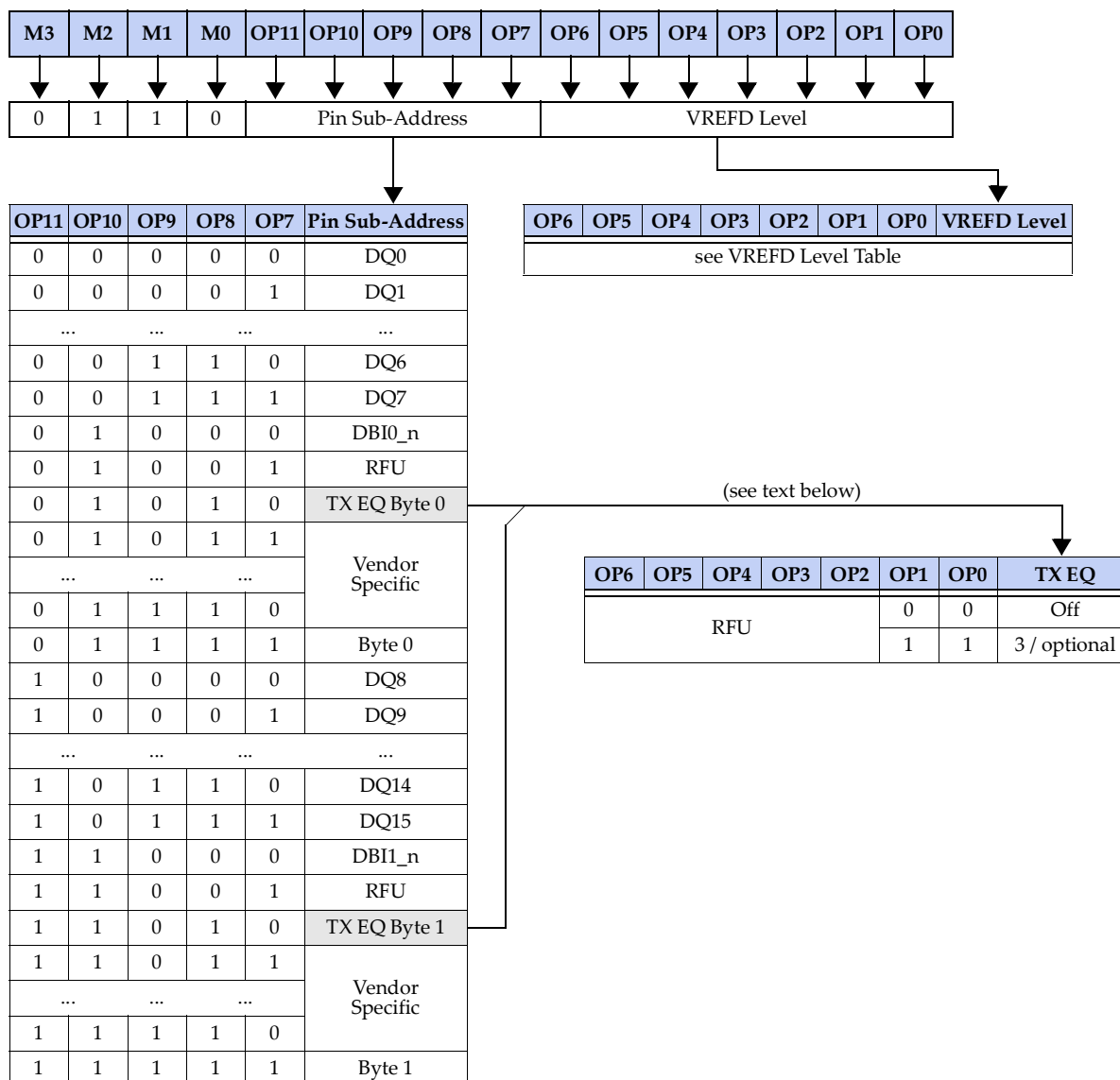
Figure 36 — Mode Register 6 (MR6) Definition
