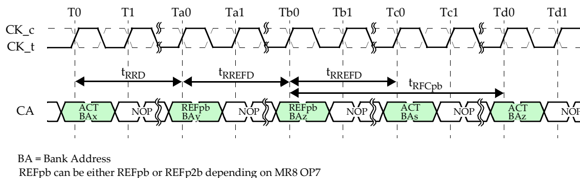
Figure 95 — REFpb / REFp2b Timings
