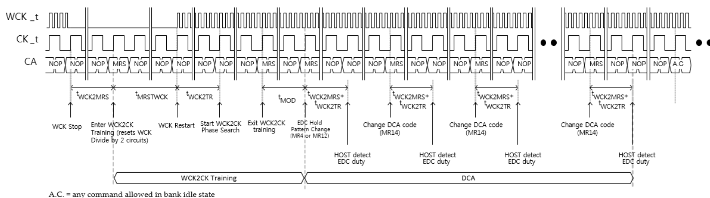
Figure 106 — DCA after WCK2CK Training
