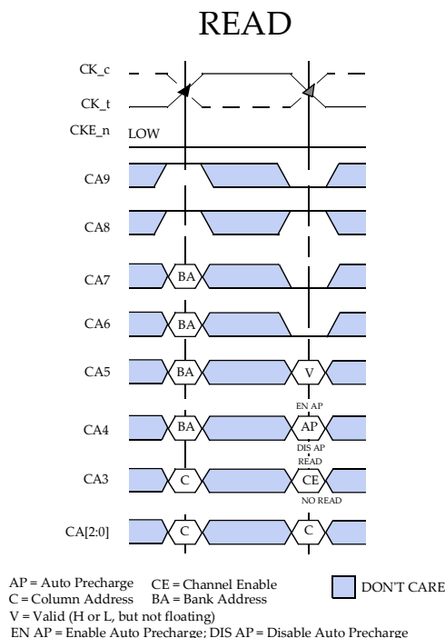
Figure 73 — READ Command
