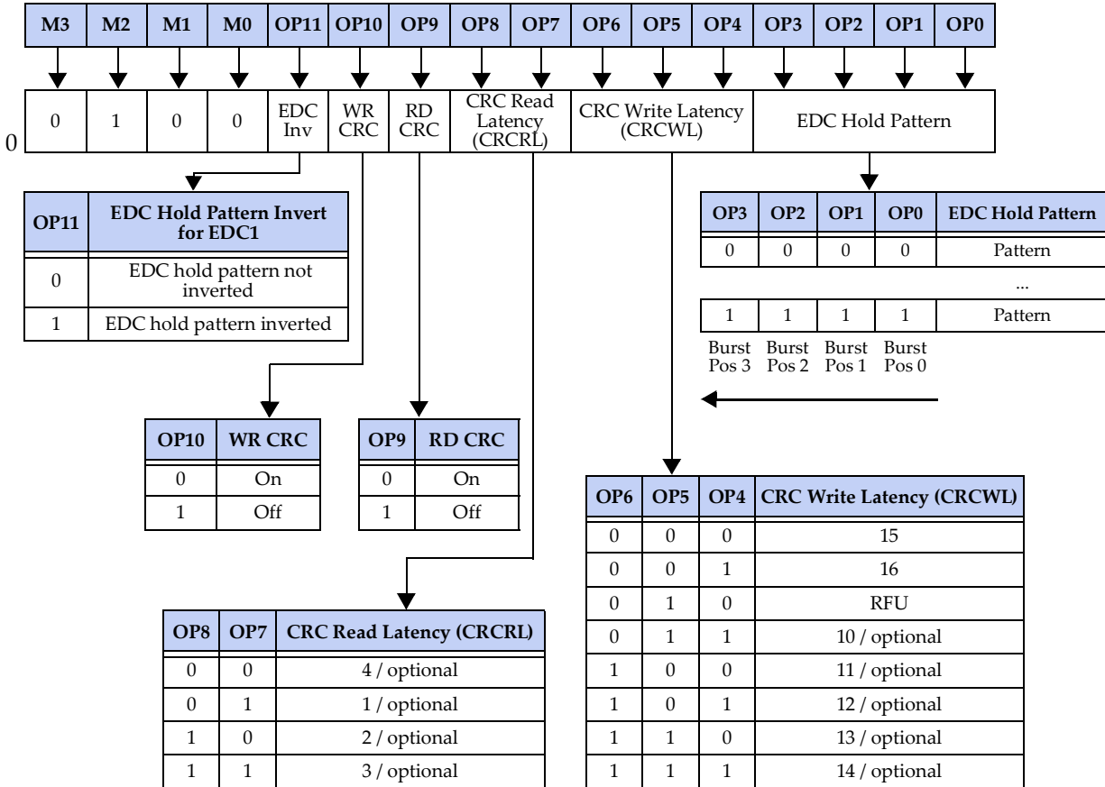
Figure 34 — Mode Register 4 (MR4) Definition
