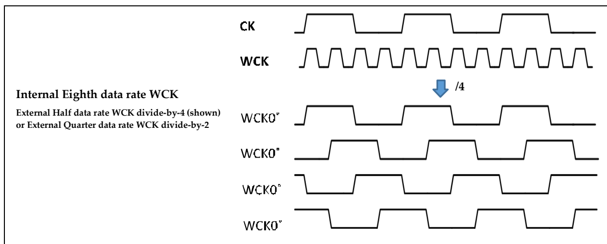
Figure 17 — Internal WCK Divider Circuit
