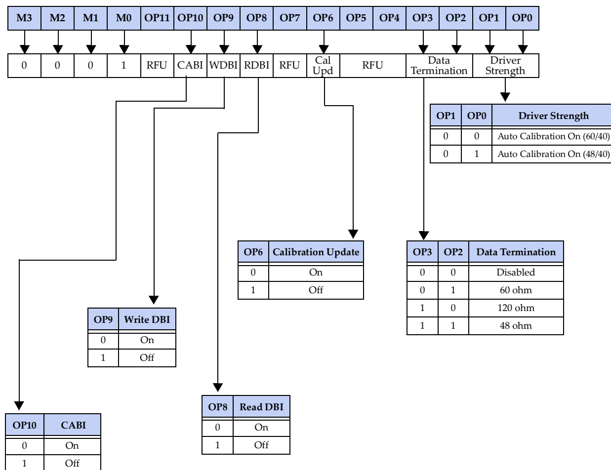
Figure 30 — Mode Register 1 (MR1) Definition
