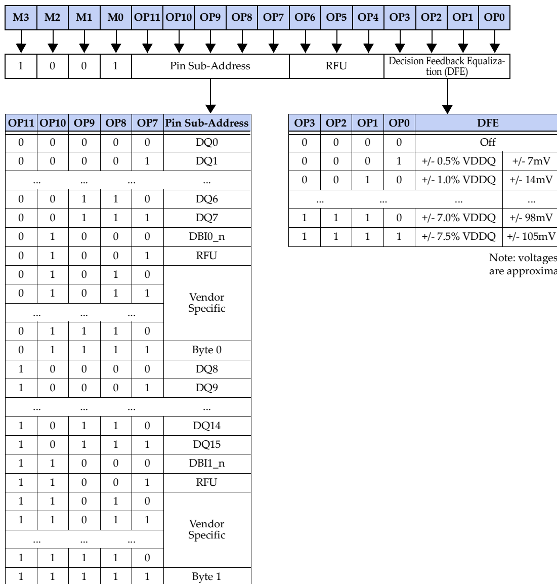
Figure 37 — Mode Register 9 (MR9) Definition
