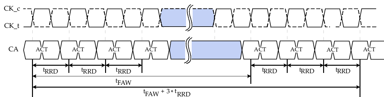
Figure 57 — t_{RRD} and t_{FAW}
