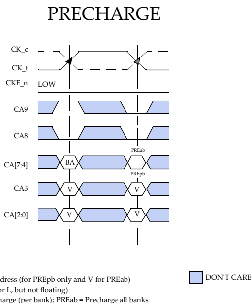
Figure 90 — PRECHARGE command
