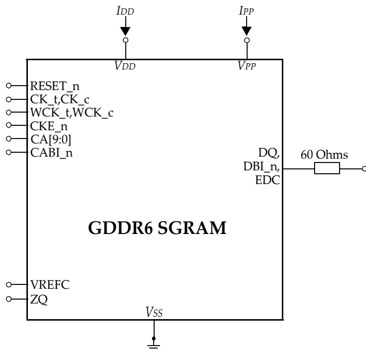
Figure 115 — Measurement Setup and Test Load for IDD and IPP Measurements
