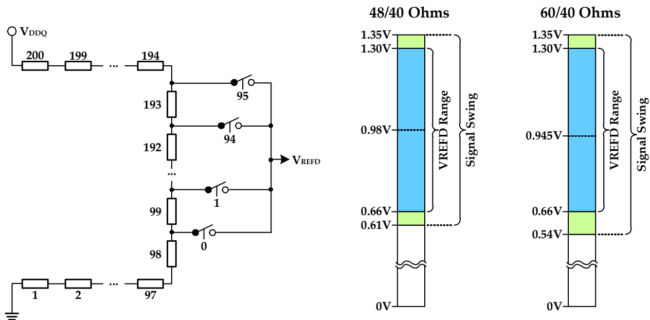
Figure 39 — VREFD Circuit and Range
