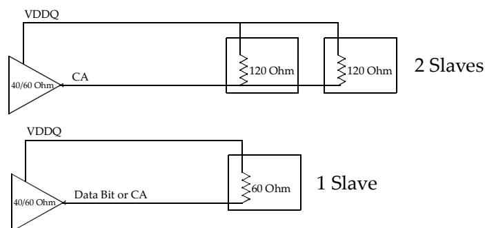
Figure 110 — System Configurations
