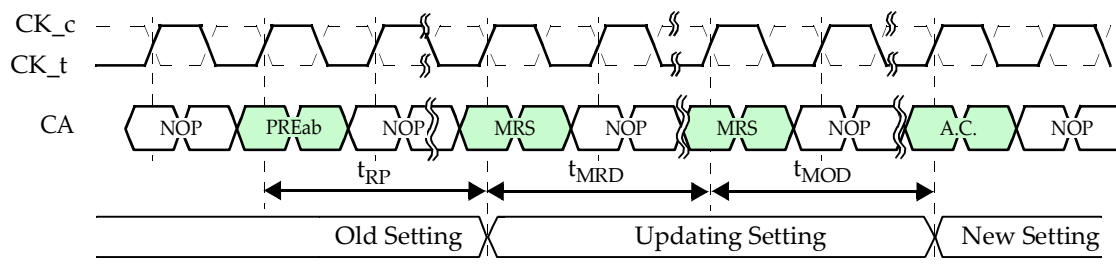
Figure 54 — Mode Register Set Timings
