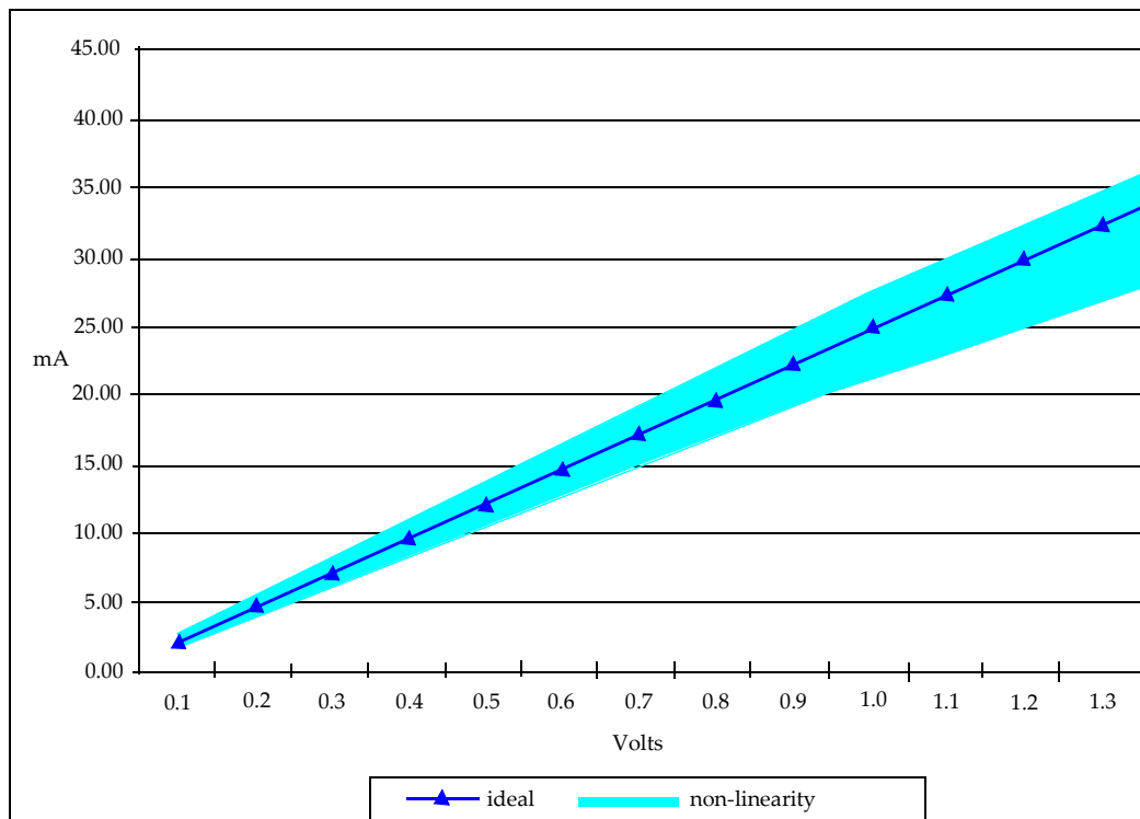
Figure 119 — Example of Non Linearity, Pull Down Characteristic at 40 ohms
