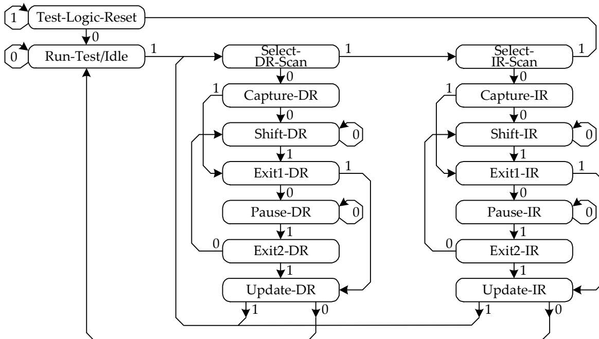
Figure 133 — TAP Controller
