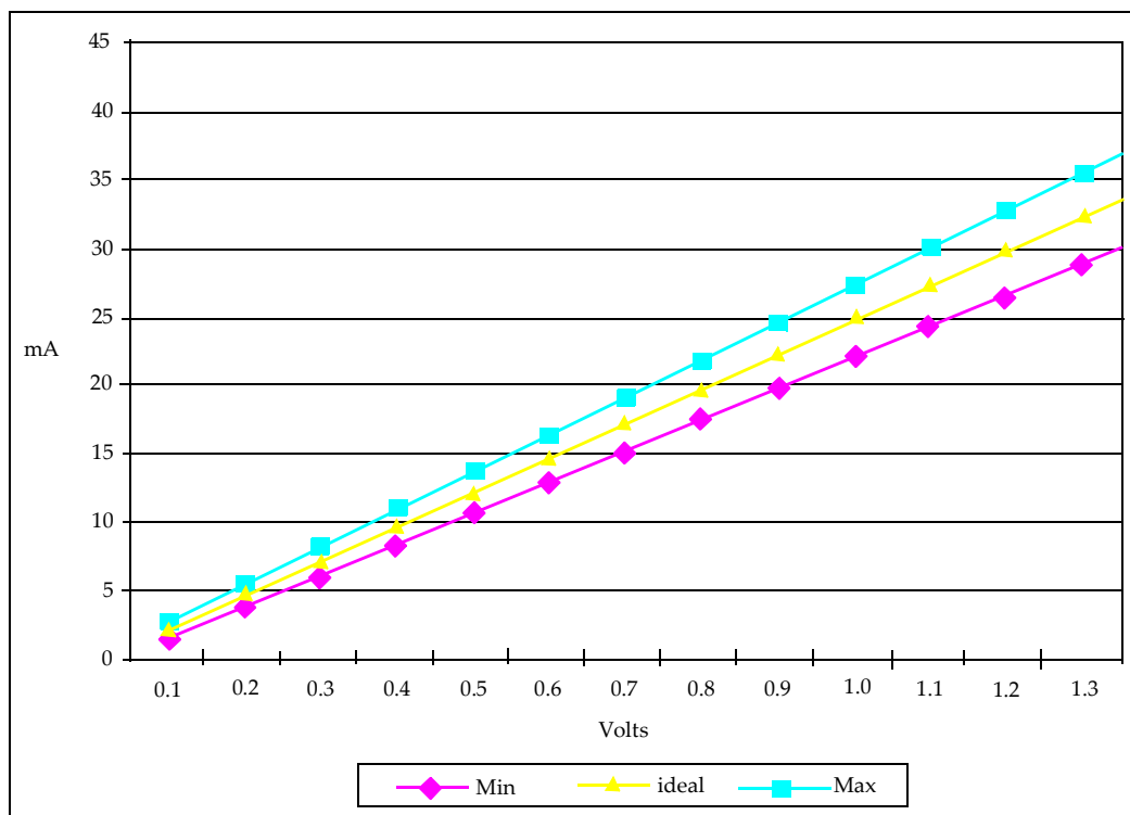
Figure 117 — Target Pull Down Characteristic at 40 ohms
