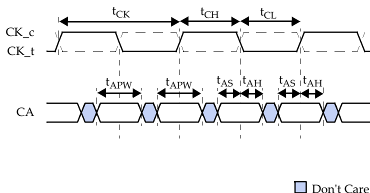
Figure 51 — Command and Address Input Timings
