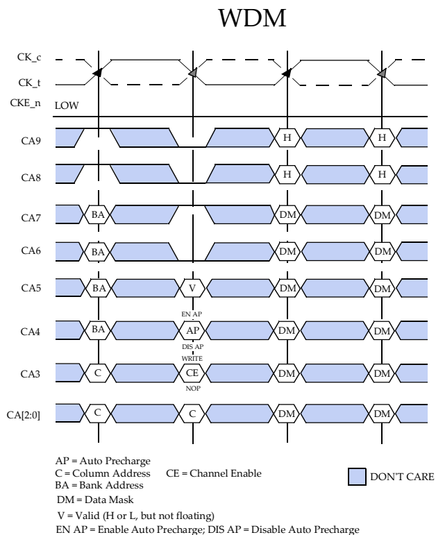
Figure 68 — WRITE-With-Doublebyte-Mask Command
