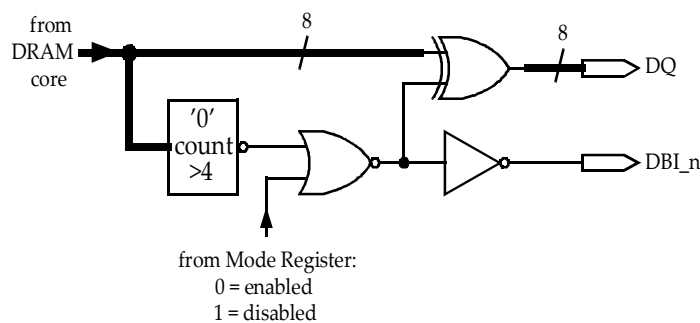
Figure 86 — Example of Data Bus Inversion Logic for READS
