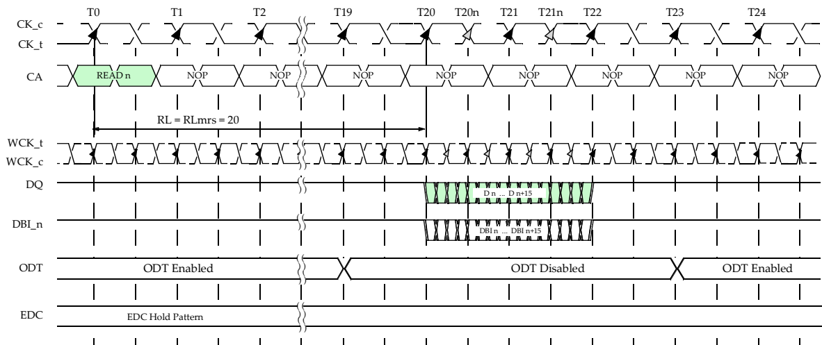
Figure 75 — Single READ without EDC (WCK DDR mode)
