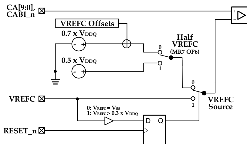
Figure 44 — VREFC Options
