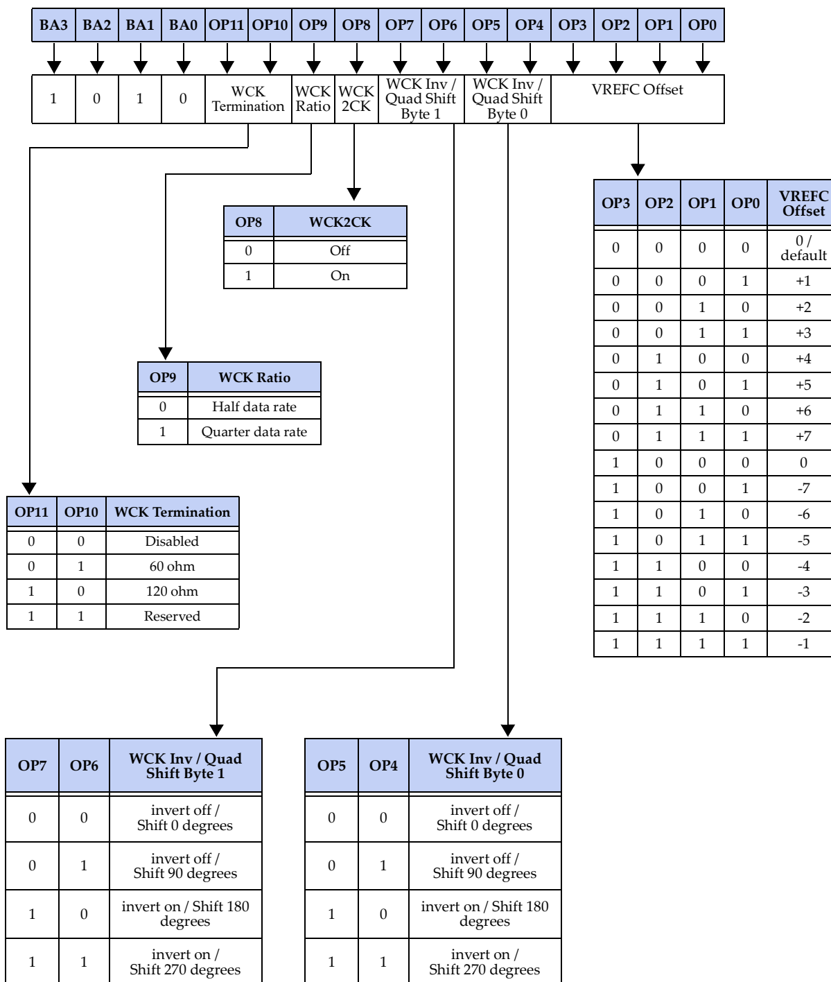
Figure 43 — Mode Register 10 (MR10) Definition
