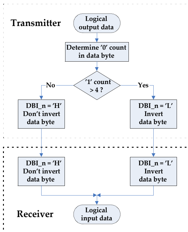
Figure 88 — DBI Flow Diagram
