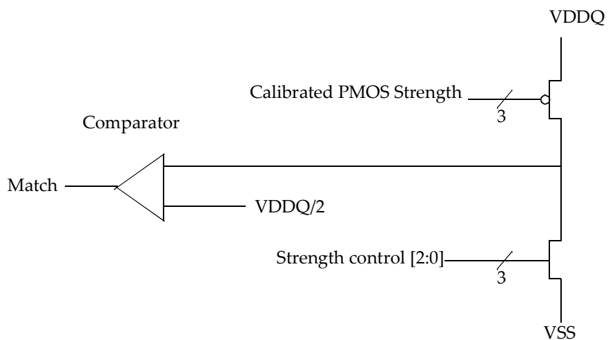
Figure 114 — NMOS Calibration
