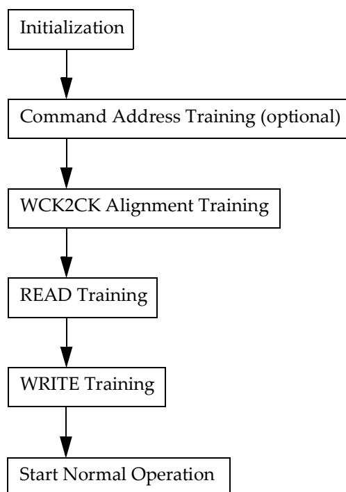
Figure 9 — Interface Training Sequence
