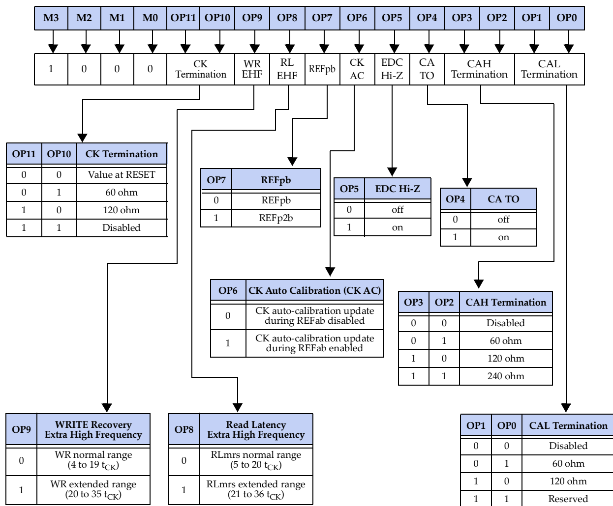
Figure 42 — Mode Register 8 (MR8) Definition
