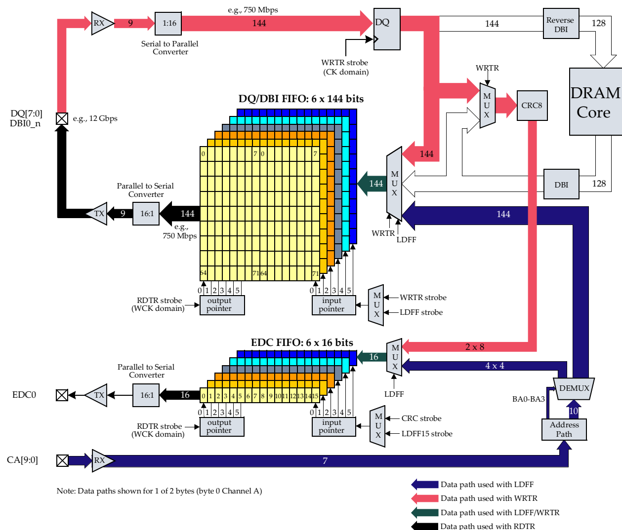
Figure 22 — Data Paths used for Read and Write Training
