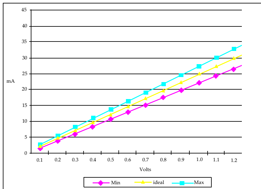
Figure 121 — Target Pull Down Characteristic at 40 ohms
