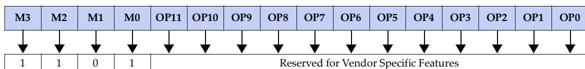
Figure 47 — Mode Register 13 (MR13) Definition
