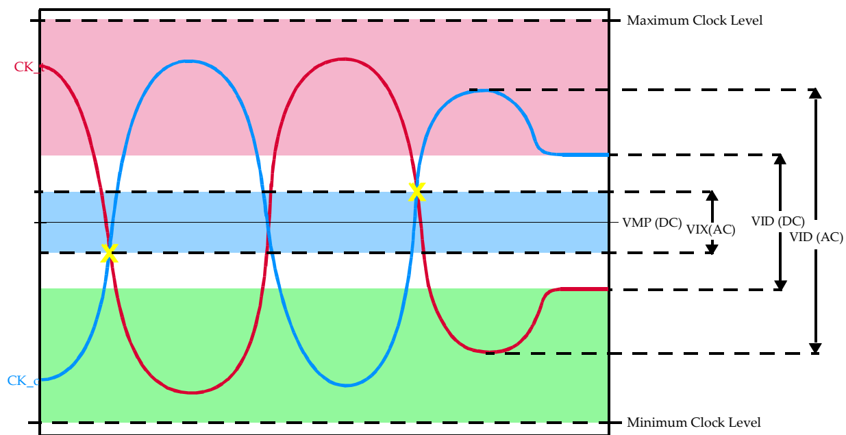
Figure 108 — Clock Waveform
