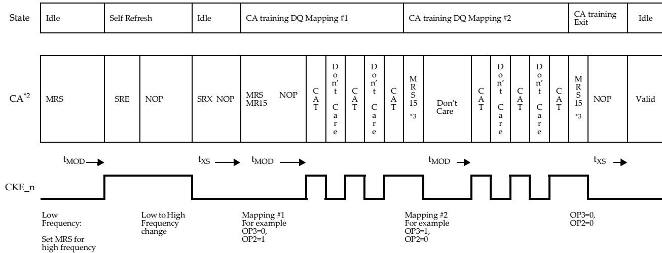
Figure 12 — Example of CACT Self Refresh - Multi pass
