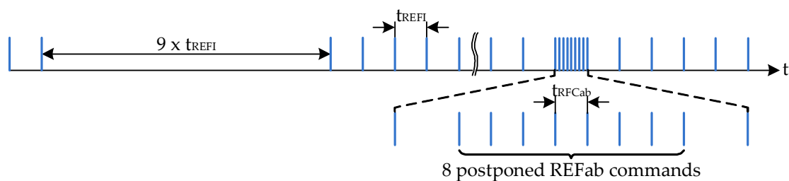
Figure 93 — Postponing REFab Commands (Example)
