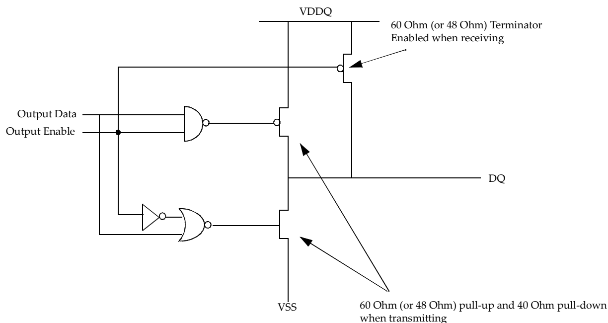
Figure 111 — Master I/O Cell
