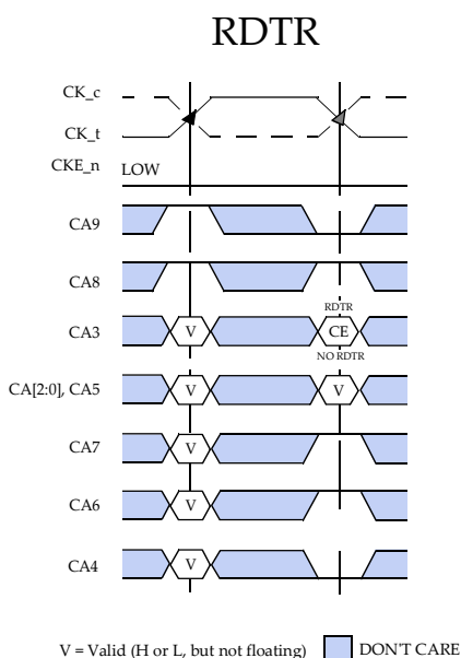
Figure 25 — RDTR Command
