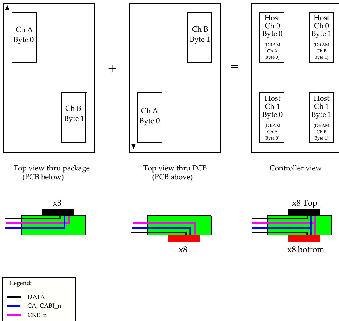
Figure 129 — Byte Orientation in Clamshell Topology
