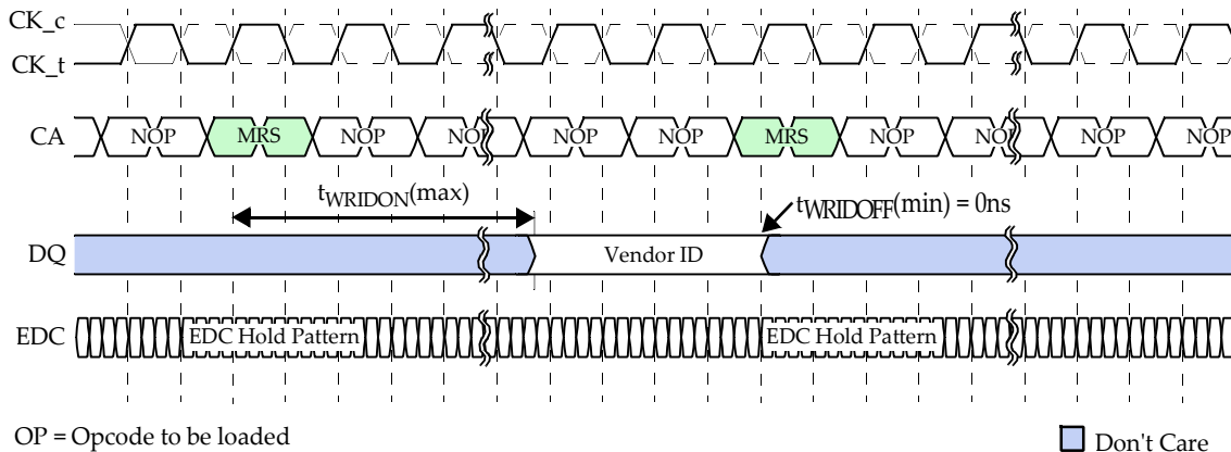
Figure 5 — Vendor ID Timing Diagram
