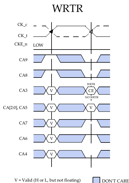
Figure 26 — WRTR Command
