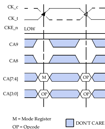
Figure 53 — MRS Command
