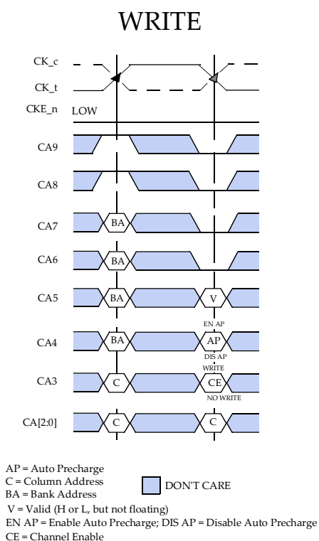
Figure 58 — WRITE Command
