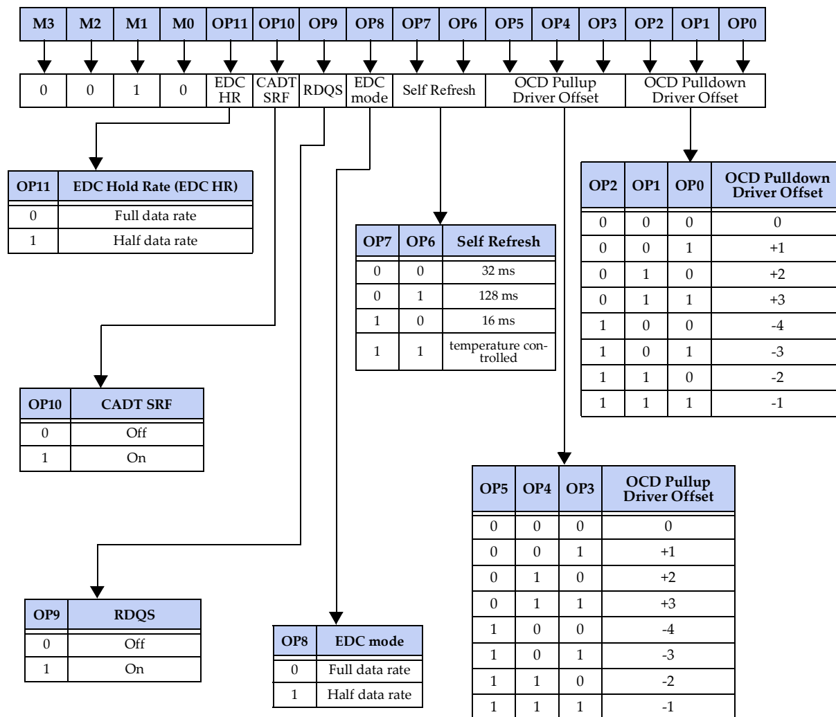
Figure 31 — Mode Register 2 (MR2) Definition
