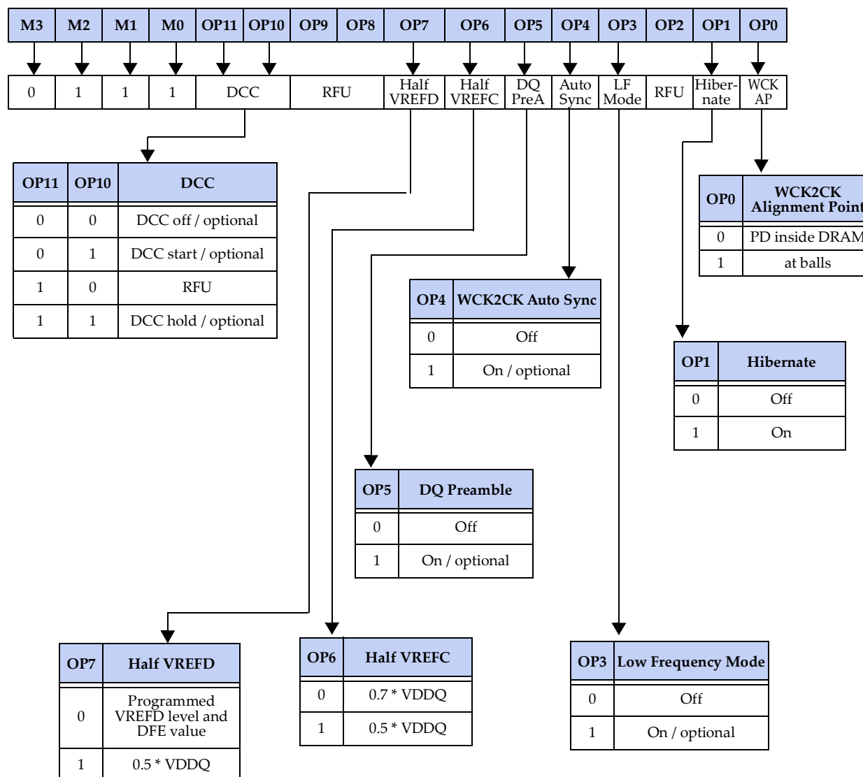
Figure 41 — Mode Register 7 (MR7) Definition
