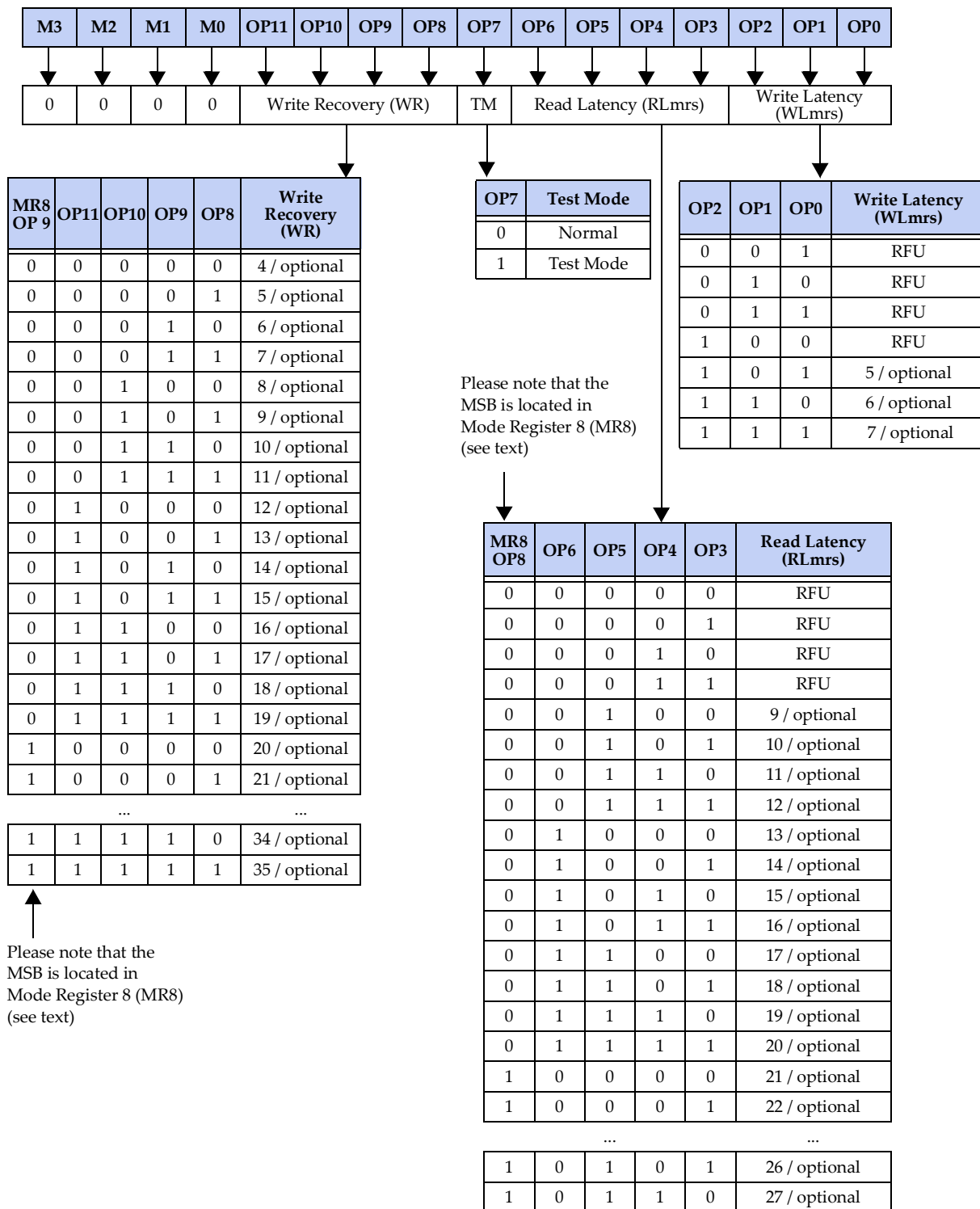
Figure 29 — Mode Register 0 (MR0) Definition
