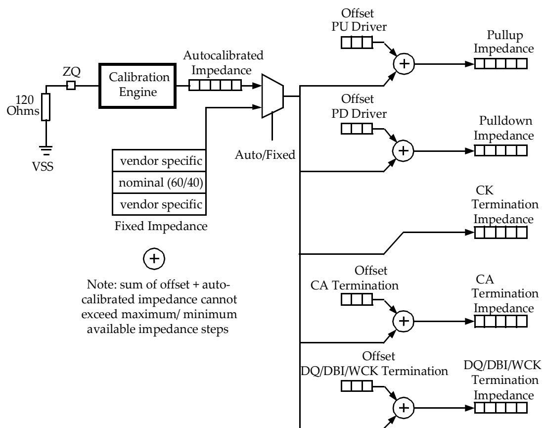
Figure 32 — Impedance Offsets
