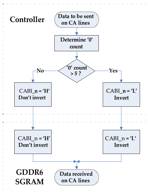
Figure 7 — Command Address Bus Inversion (CABI) Flow Diagram
