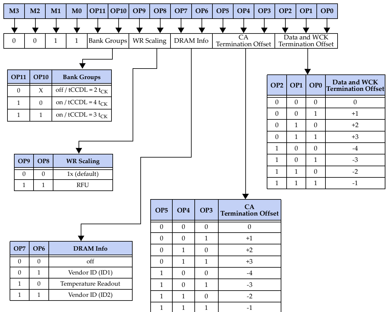
Figure 33 — Mode Register 3 (MR3) Definition
