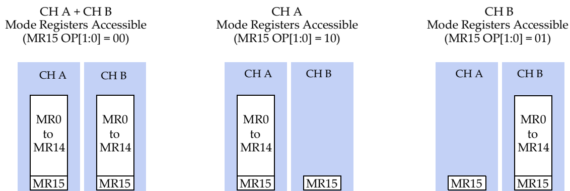
Figure 50 — Mode Register Enable
