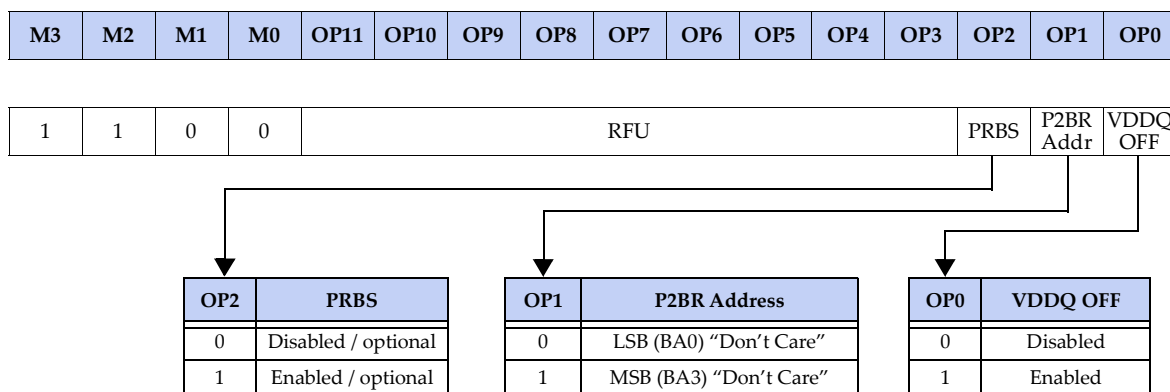
Figure 46 — Mode Register 12 (MR12) Definition
