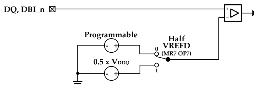
Figure 38 — VREFD Options
