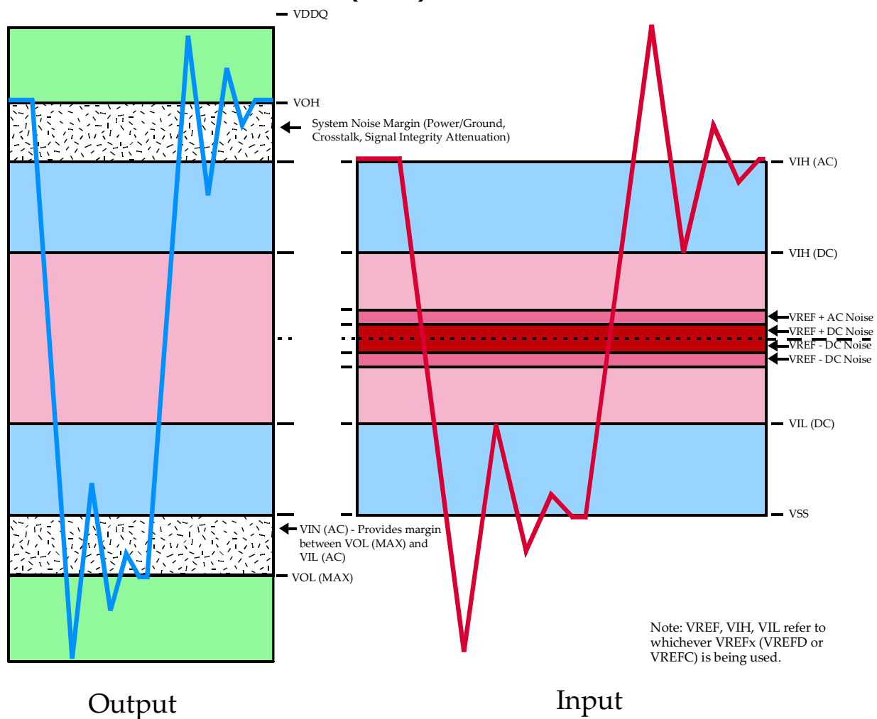
Figure 107 — Voltage Waveform
