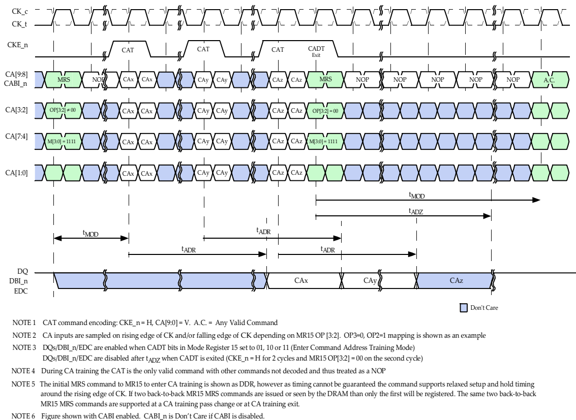
Figure 10 — Command Address Training Timing - Single Pass
