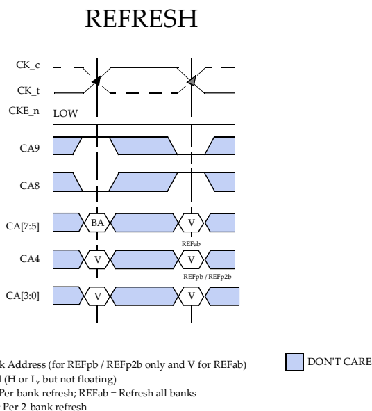
Figure 91 — REFRESH Command
