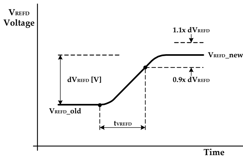
Figure 40 — VREFD and DFE Settling Time
