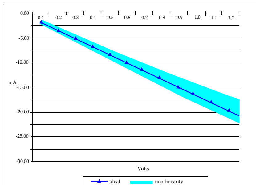
Figure 124 — Example of Non Linearity, Pull Up/Termination Characteristic at 60 ohms
