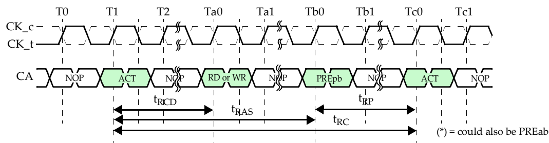
Figure 55 — ACTIVATE Command
