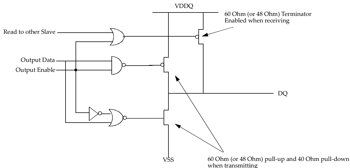
Figure 112 — Slave I/O Cell
