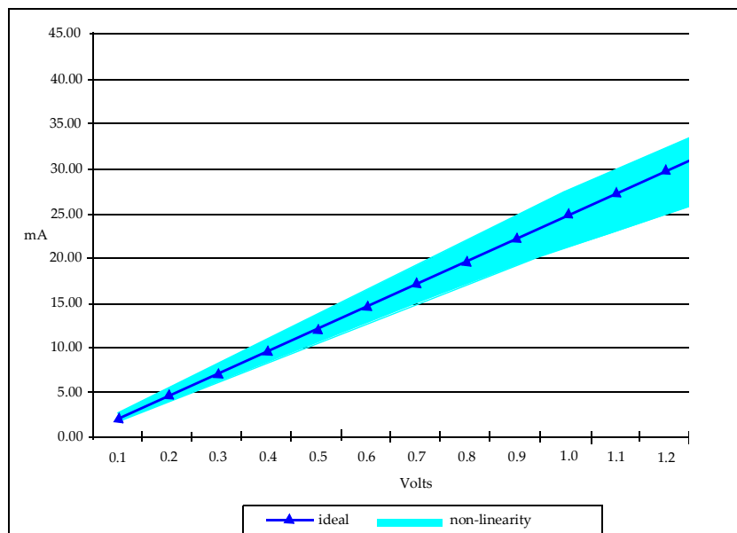
Figure 123 — Example of Non Linearity, Pull Down Characteristic at 40 ohms
