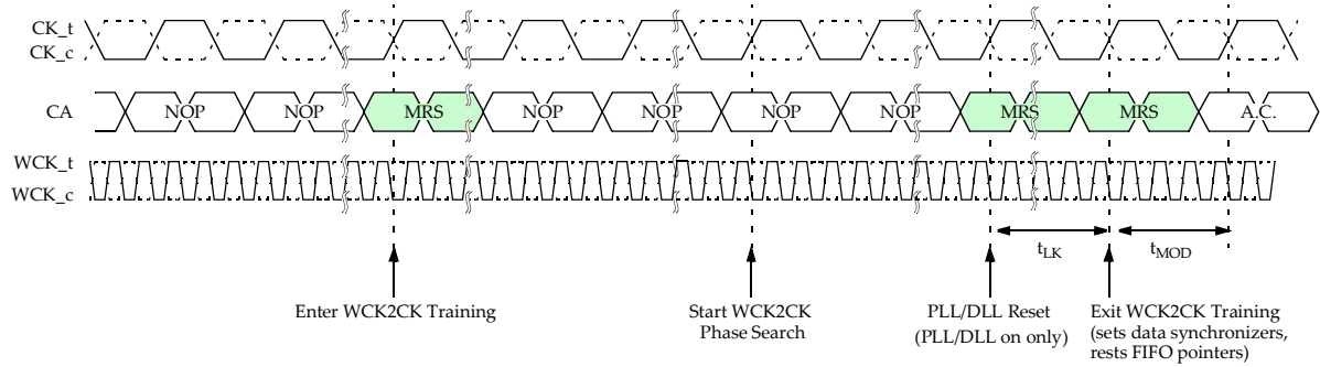
Figure 14 — Example WCK2CK Training Sequence
