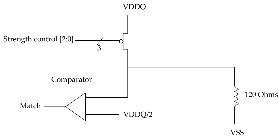
Figure 113 — PMOS Calibration
