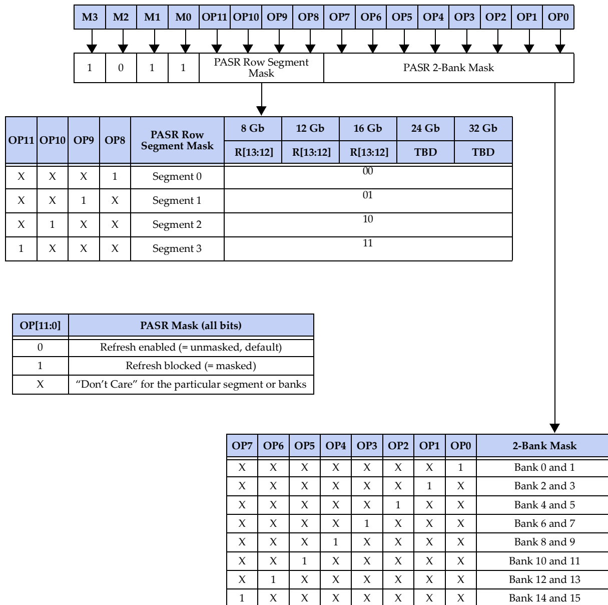
Figure 45 — Mode Register 11 (MR11) Definition
