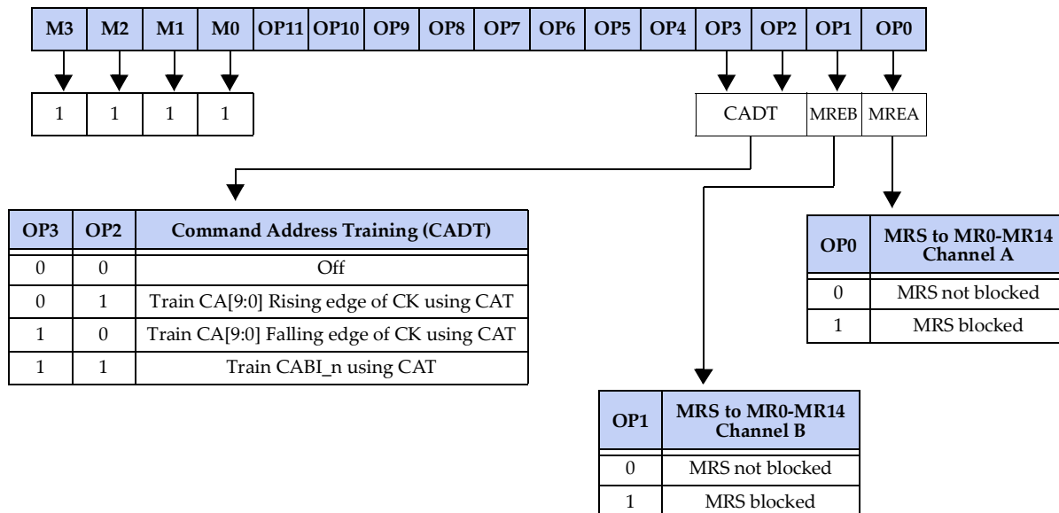
Figure 49 — Mode Register 15 (MR15) Definition
