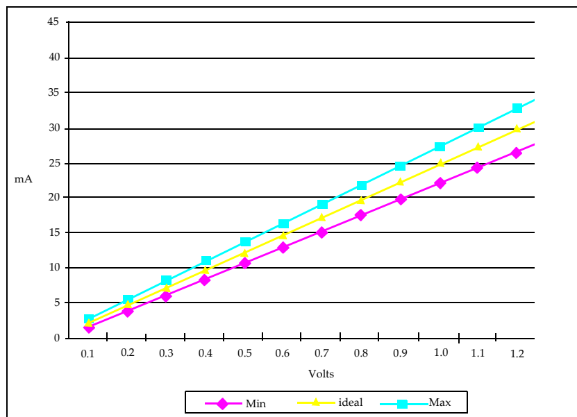
Figure 122 — Target Pull Up/Termination Characteristic at 60 ohms
