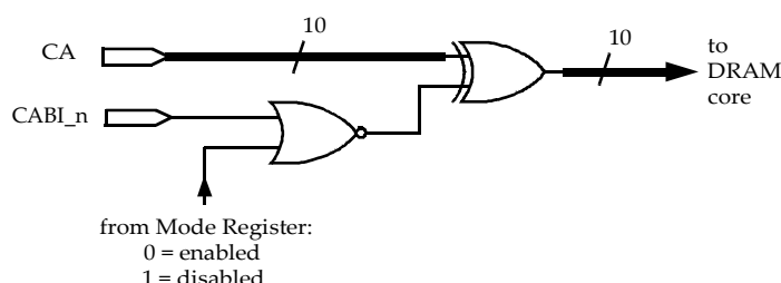
Figure 6 — Example of Command Address Bus Inversion Logic
