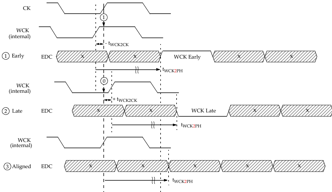
Figure 15 — Example WCK2CK Training Sequence with WCK Stopping
