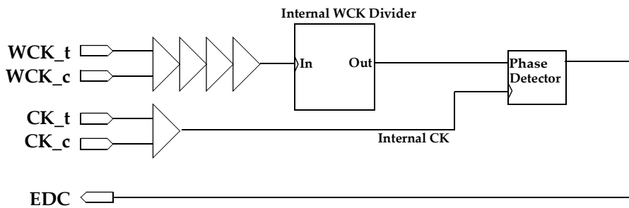
Figure 18 — Normal Mode
