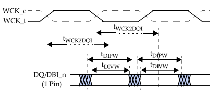
Figure 52 — Data Input Timings
