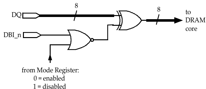
Figure 87 — Example of Data Bus Inversion Logic for WRITES
