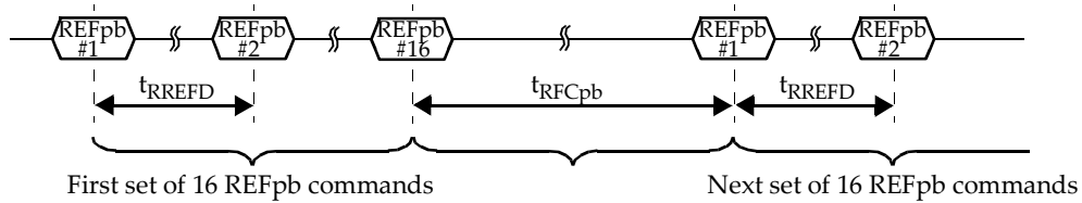
Figure 96 — Sets of REFpb Commands
