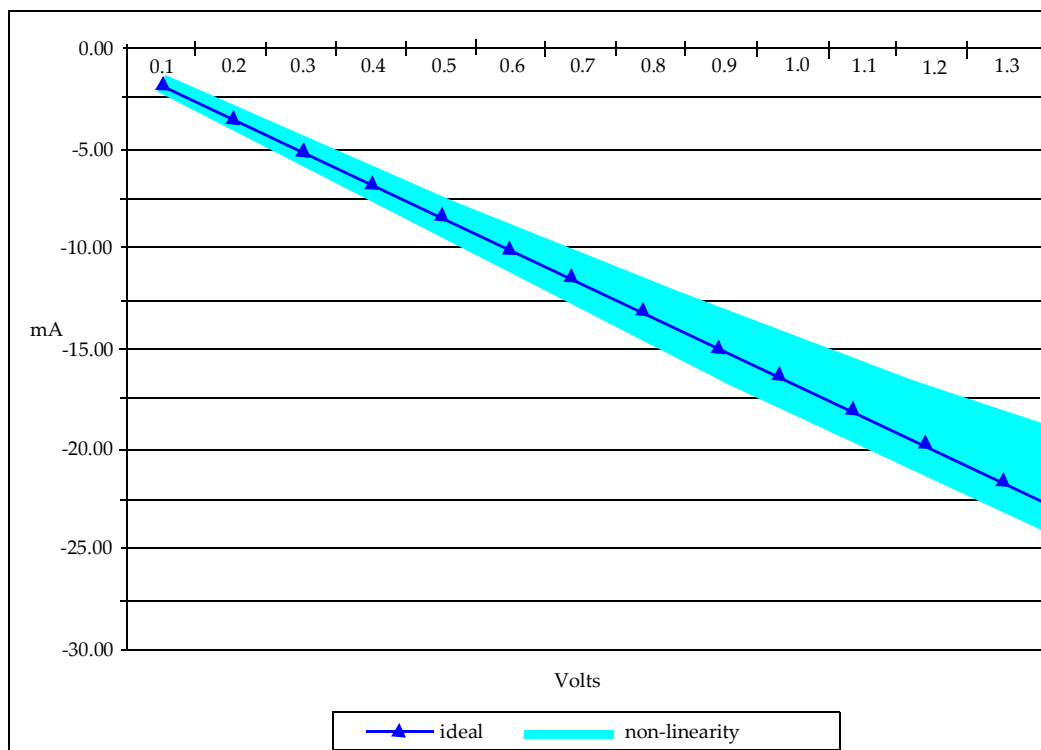
Figure 120 — Example of Non Linearity, Pull Up/Termination Characteristic at 60 ohms
