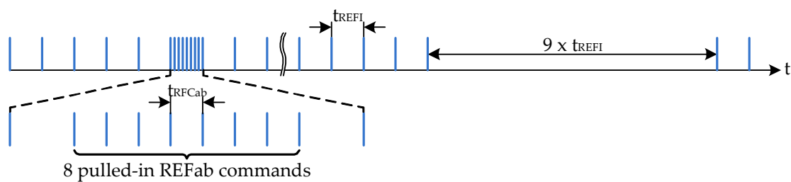
Figure 94 — Pulling-In REFab Commands (Example)
