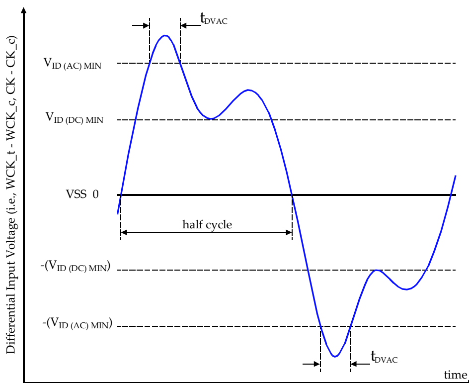
Figure 109 — Definition of differential ac-swing and "time above ac-level" t_{DVAC}
