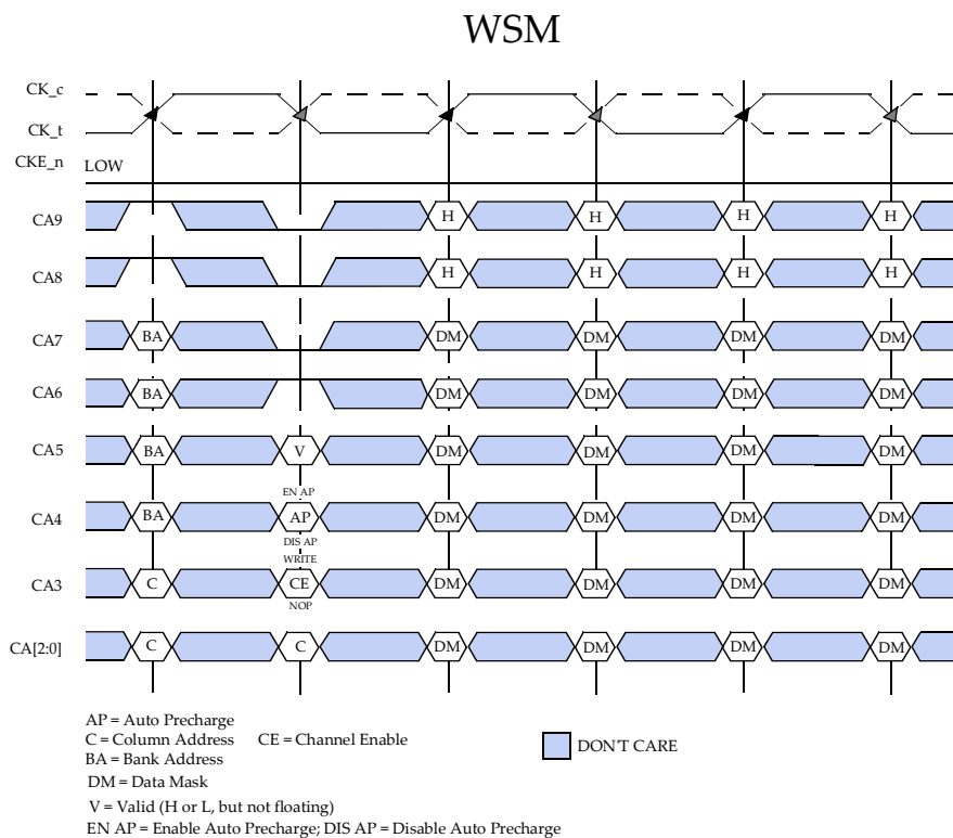
Figure 70 — WRITE-With-Singlebyte-Mask Command
