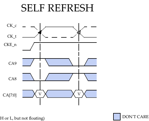
Figure 98 — SELF REFRESH Entry Command
