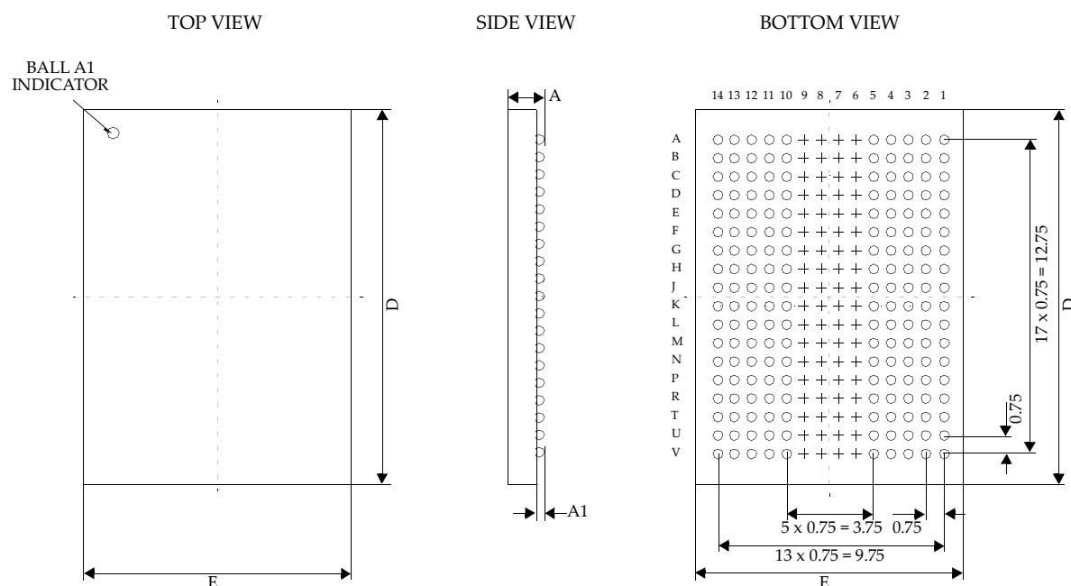
Figure 126 — Package Dimensions 2
