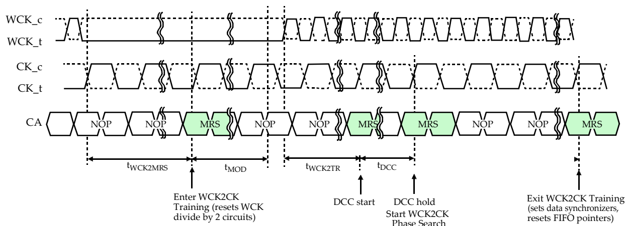
Figure 105 — WK2CK Training Sequence with DCC
