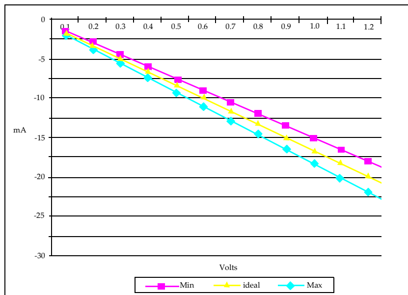
Figure 118 — Target Pull Up/Termination Characteristic at 60 ohms
