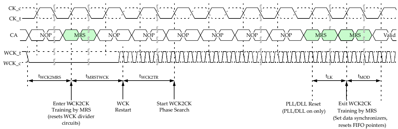
Figure 15 — Example WCK2CK Training Sequence with WCK Stopping
