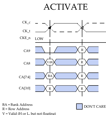
Figure 55 — ACTIVATE Command
