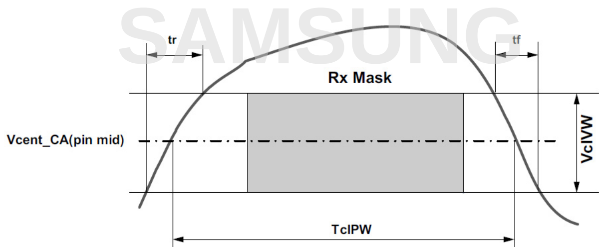
Figure 29. CA TclPW and SRIN_cIVW definition (for each input pulse)
