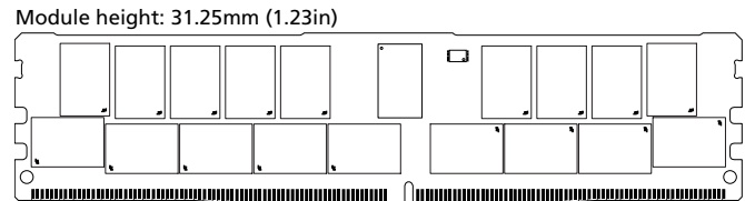
Figure 2: 288-Pin RDIMM (MO-309, R/C-B2)
