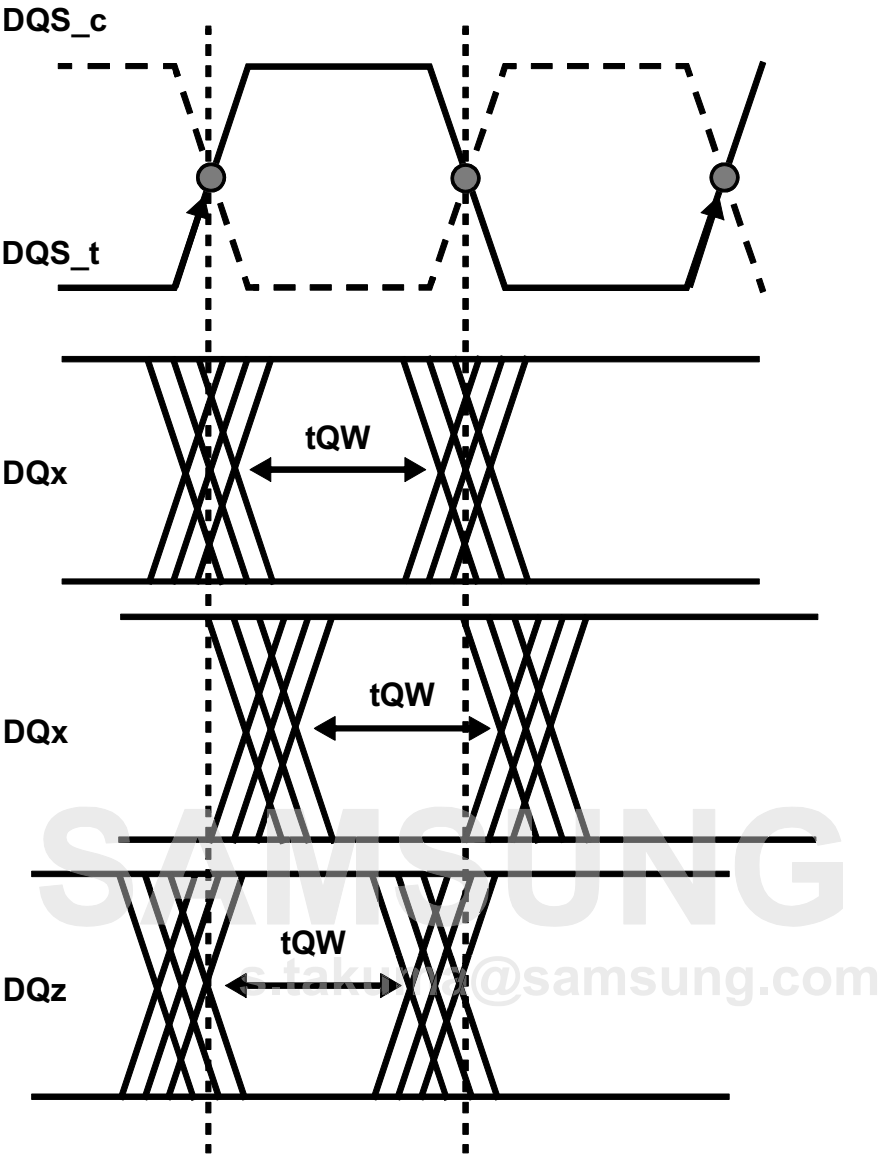
Figure 32. Read data timing tQW valid window defined per DQ signal
