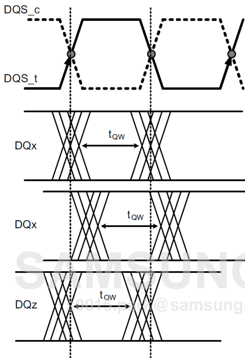
Figure 24. Read data timing t_{QW} valid window defined per DQ signal
