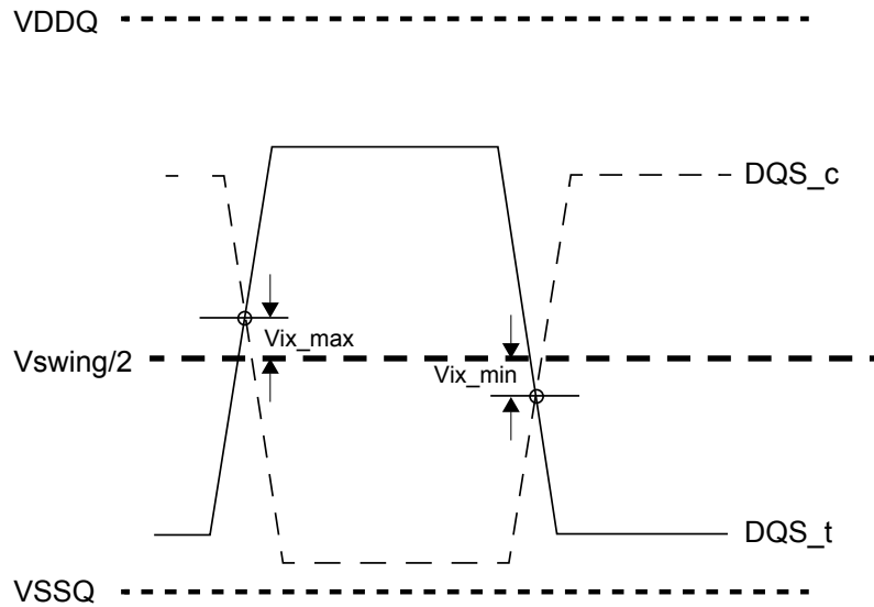
Figure 8. DQS input Crosspoint (Vix) voltage
