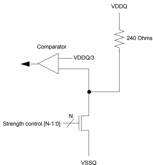
Figure 15. pull-down calibration
