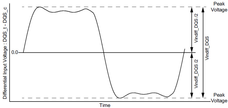
Figure 7. DQS Differential Input Voltage
