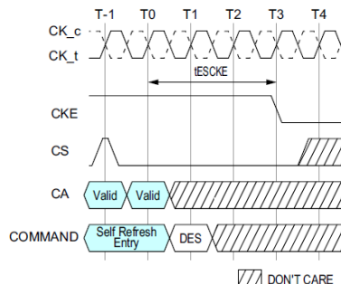
Figure 17. t CMDCKE Timing
