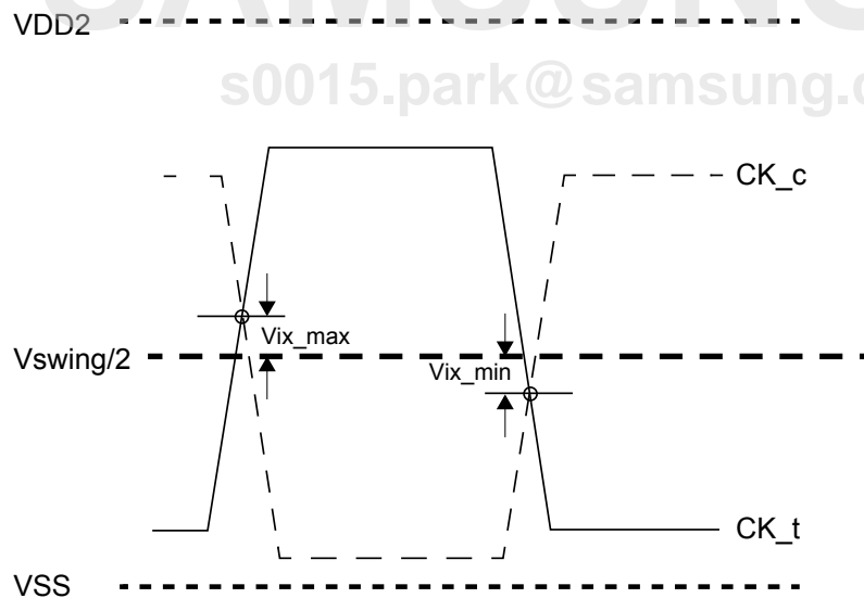
Figure 9. CK input Crosspoint voltage (Vix)
