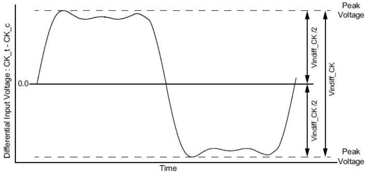
Figure — CK Differential input voltage Table
