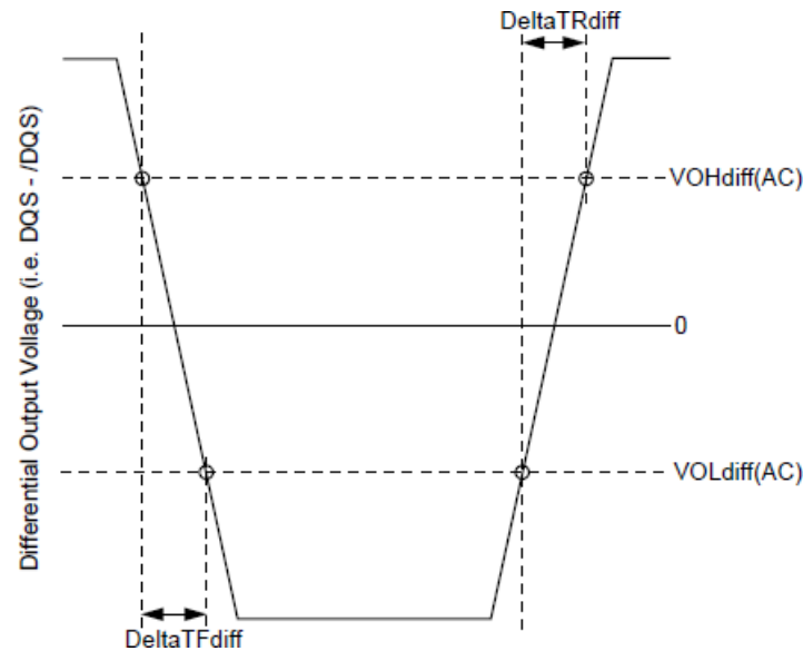
Figure — Differential Output Slew Rate
