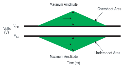
Clock, Data, Strobe, Mask Overshoot and Undershoot Definition
