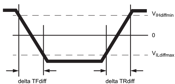
Differential Input Slew Rate definition for \overline{\text{DQS}} , \overline{\text{DQS}} , and \overline{\text{CK}} , \overline{\text{CK}}
