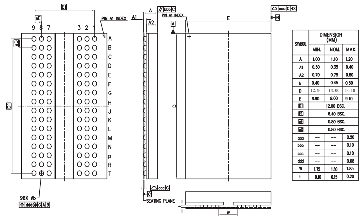
Package Diagram (x16) 96-Ball Fine Pitch Ball Grid Array Outline
