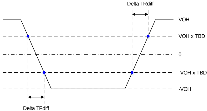
Figure 307 — Differential Output Slew Rate Definition
