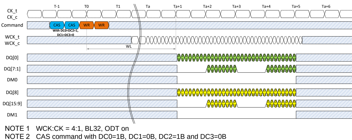
Figure 267 — Example of Write Data Copy Function Timing Diagram
