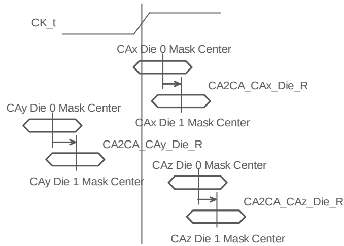
Figure 328 — CK_t Rising Edge CA Mask
