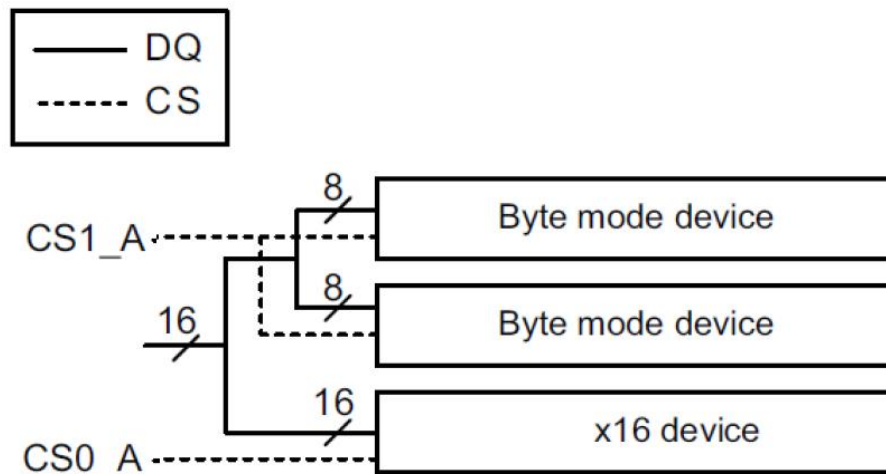
Figure 334 — Example of Rank Assignment for a Single-channel Dual-rank Package
