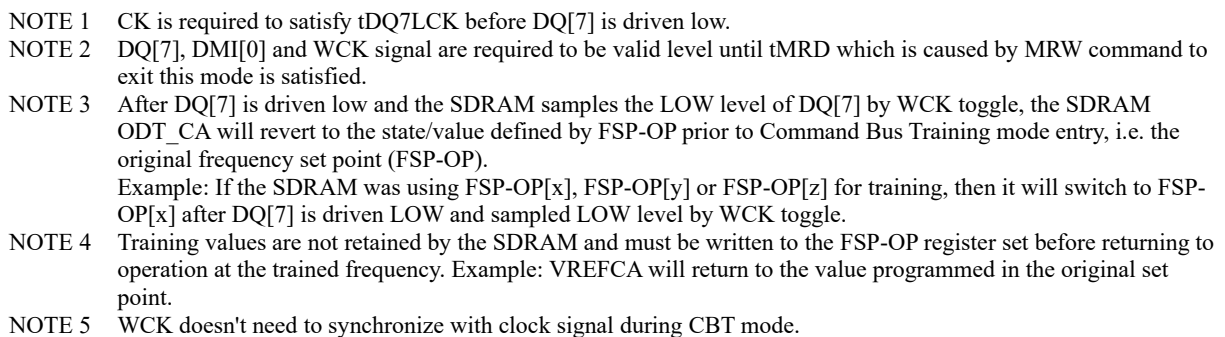
Figure 41 — Exiting Command Bus Training Mode (Command-based ZQ Calibration)
