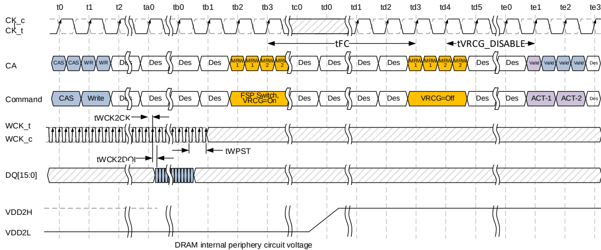
Figure 258 — DVFS Low (VDD2L) to High (VDD2H) Transition
