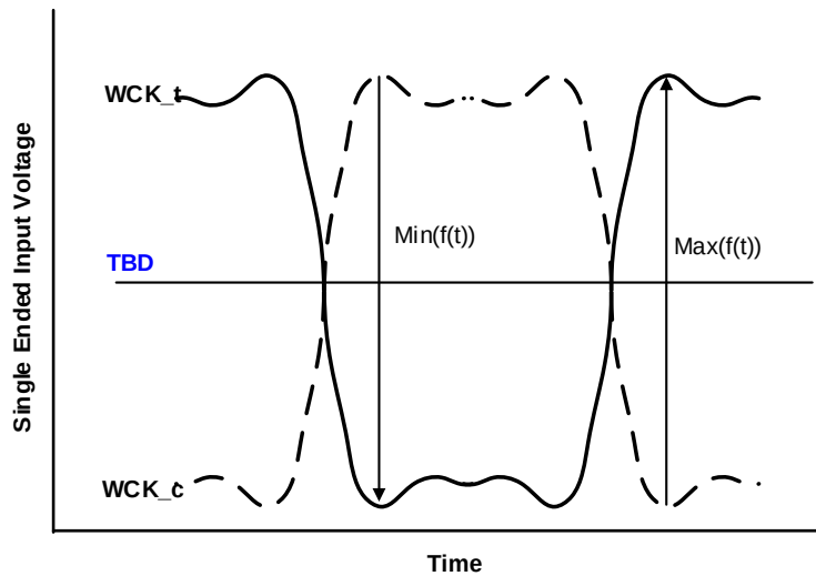
Figure 302 — Definition of Differential WCK Peak Voltage
