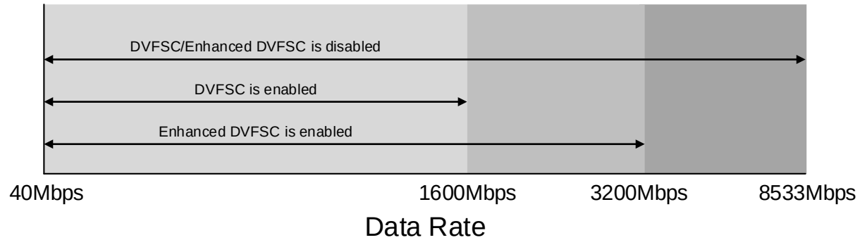
Figure 256 — The Frequency Range Supported by DVFSC and Enhanced DVFSC Mode
