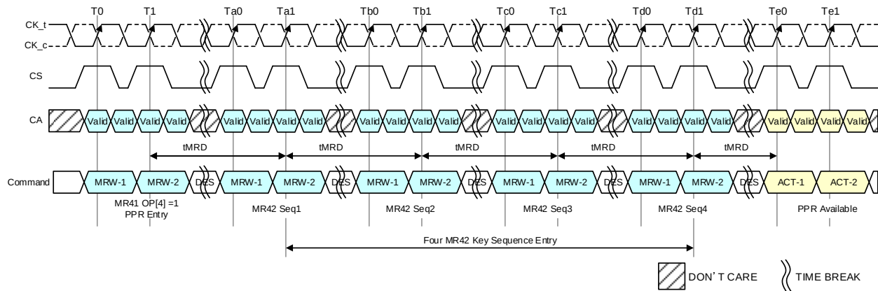
Figure 274 — Guard Key Timing Diagram
