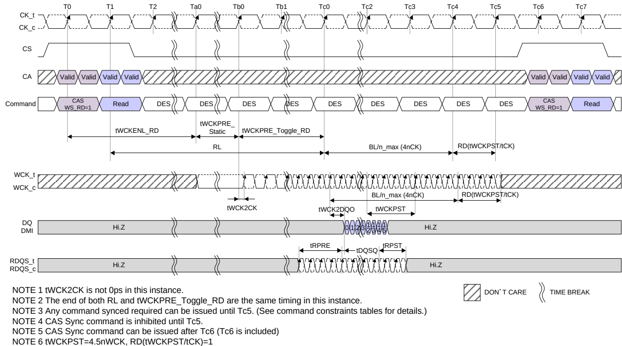
Figure 85 — Read Sync Off Timing (WCK2CK Sync is Expired) BG Mode, CKR=4:1, BL=16, t_{RPST}=2.5nWCK
