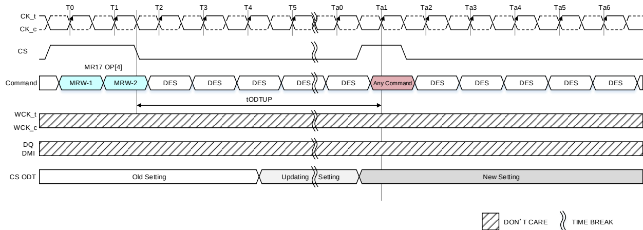
Figure 209 — ODT for CS Setting Update Timing
