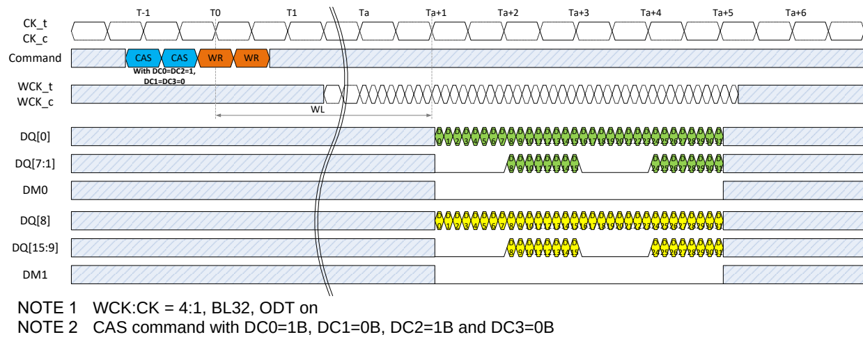
Figure 267 — Example of Write Data Copy Function Timing Diagram
