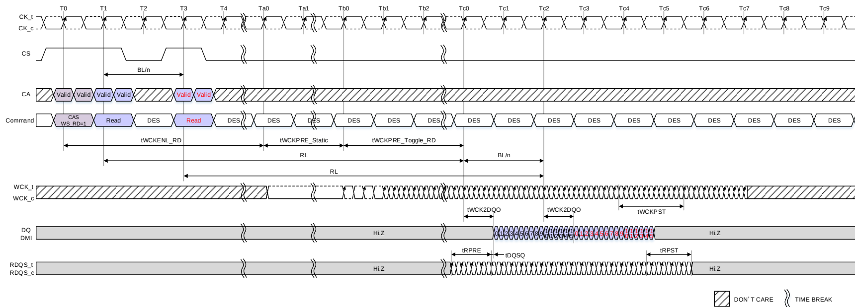
Figure 107 — Back to Back Read Operation with BL/n, BG Mode, CKR = 4:1, tRPST = 4.5tWCK, tWCKPST = 6.5tWCK
