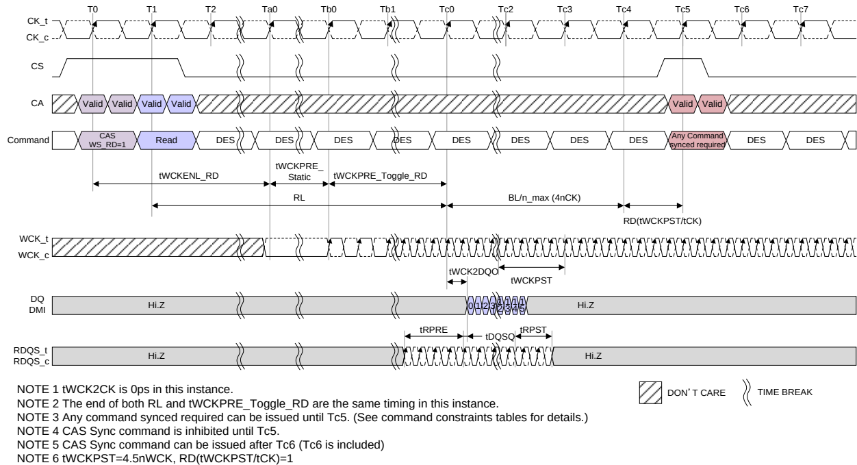
Figure 84 — Read Sync Off Timing BG Mode : CKR (WCK vs. CK = 4:1, BL=16, t_{RPST}=2.5nWCK
