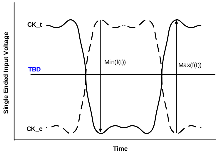
Figure 297 — Definition of Differential Clock Peak Voltage
