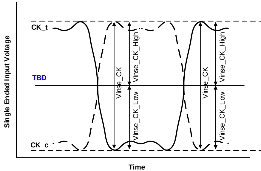
Figure 298 — Clock Single-ended Input Voltage
