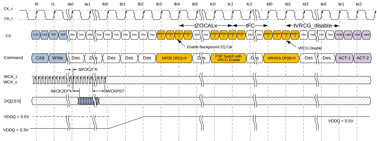
Figure 263 — DVFSQ Low (VDDQ) to High Transition Timing without VRCG during VddQ Ramp
