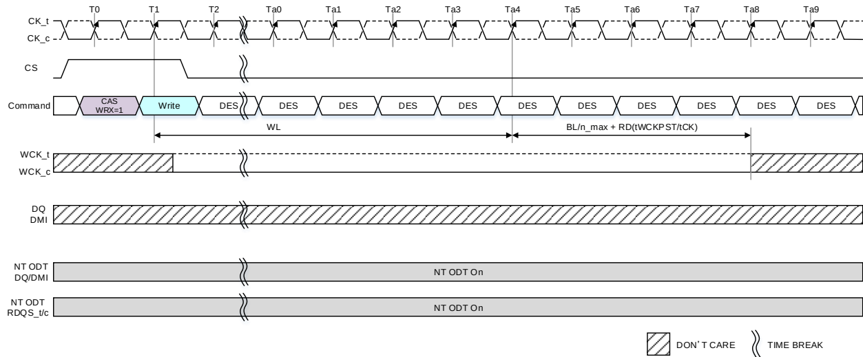
Figure 231 — NT ODT Timing at Write X for Write BG Mode: CKR (WCK vs. CK) = 4:1, BL=16
