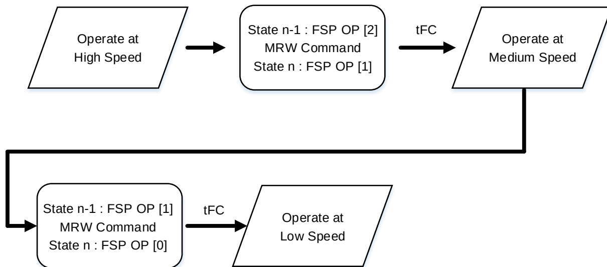
Figure 205 — Switching to a Third Trained Frequency Set-Point (Example)
