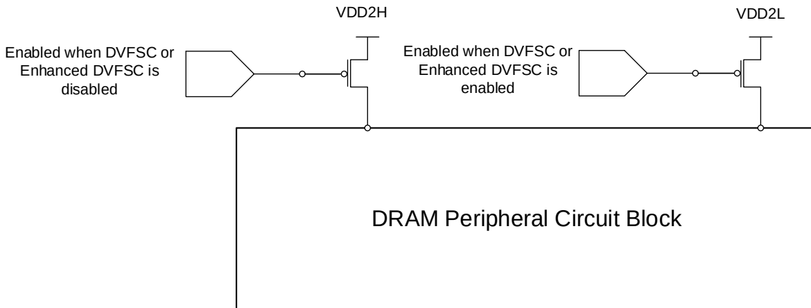
Figure 259 — Example DVFS/Enhanced DVFS Block Diagram
