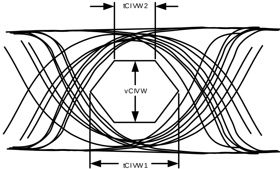
Figure 325 — CA Rx Mask Definition
