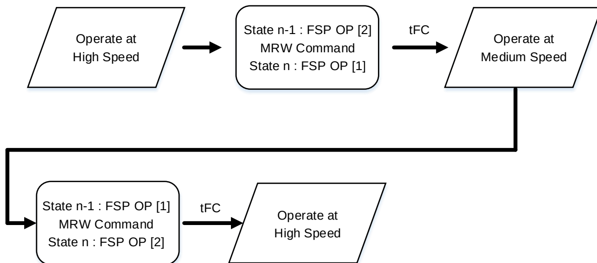
Figure 204 — Switching Between Two Trained Frequency Set-Points (Example)
