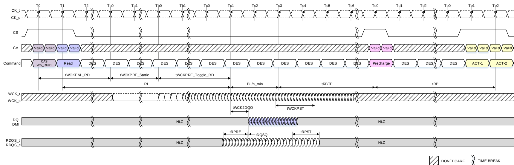
Figure 106 — Burst Read Operation: BG Mode, CKR=4:1
