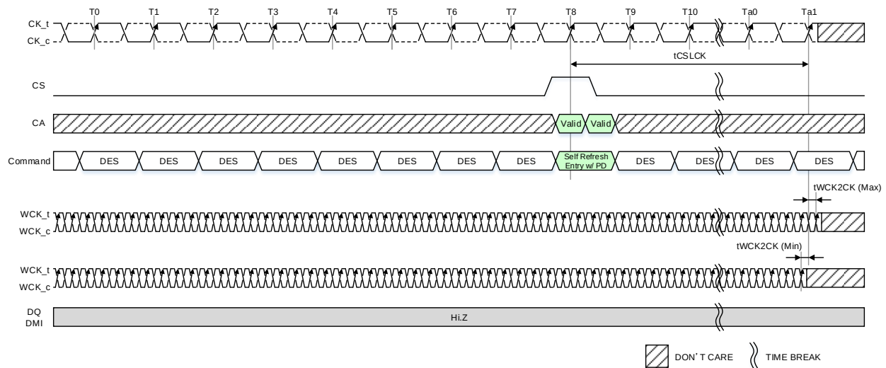
Figure 187 — Self Refresh with Power Down Entry to CK and WCK Stop Timing
