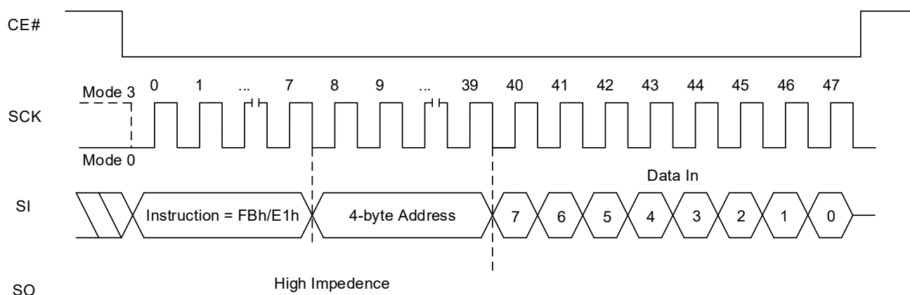
Figure 8.120 Write DYB Sequence In SPI Mode (FBh [EXTADD=1] or E1h, 4-byte address)
